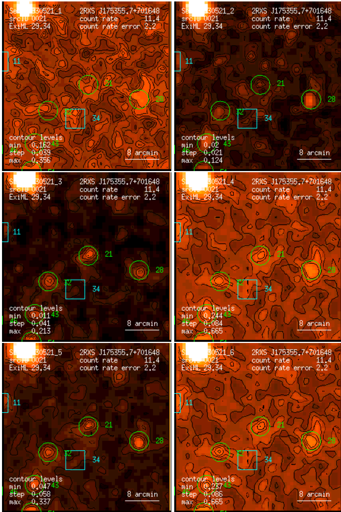
Figure 21: RASS 930521: detection 0021: band rate images, Gaussian filter: (1) PSPC channels 11 – 41, (2) 52 – 90, (3) 91 – 201, (4) 11 – 235, (5) 52 – 201, (6) 11 – 201. Broad band rates in counts/ks. Band rate contour levels in counts/ks/arcmin 2 .
