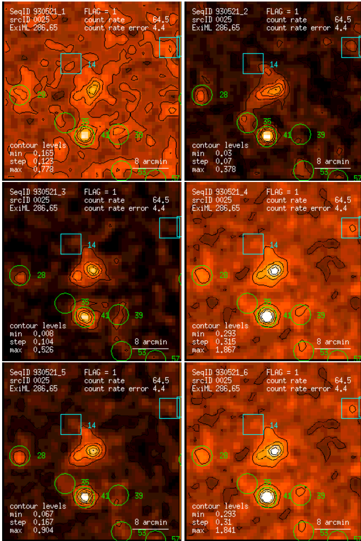
Figure 25: RASS 930521: detection 0025: band rate images, Gaussian filter: (1) PSPC channels 11 – 41, (2) 52 – 90, (3) 91 – 201, (4) 11 – 235, (5) 52 – 201, (6) 11 – 201. Broad band rates in counts/ks. Band rate contour levels in counts/ks/arcmin 2 .
