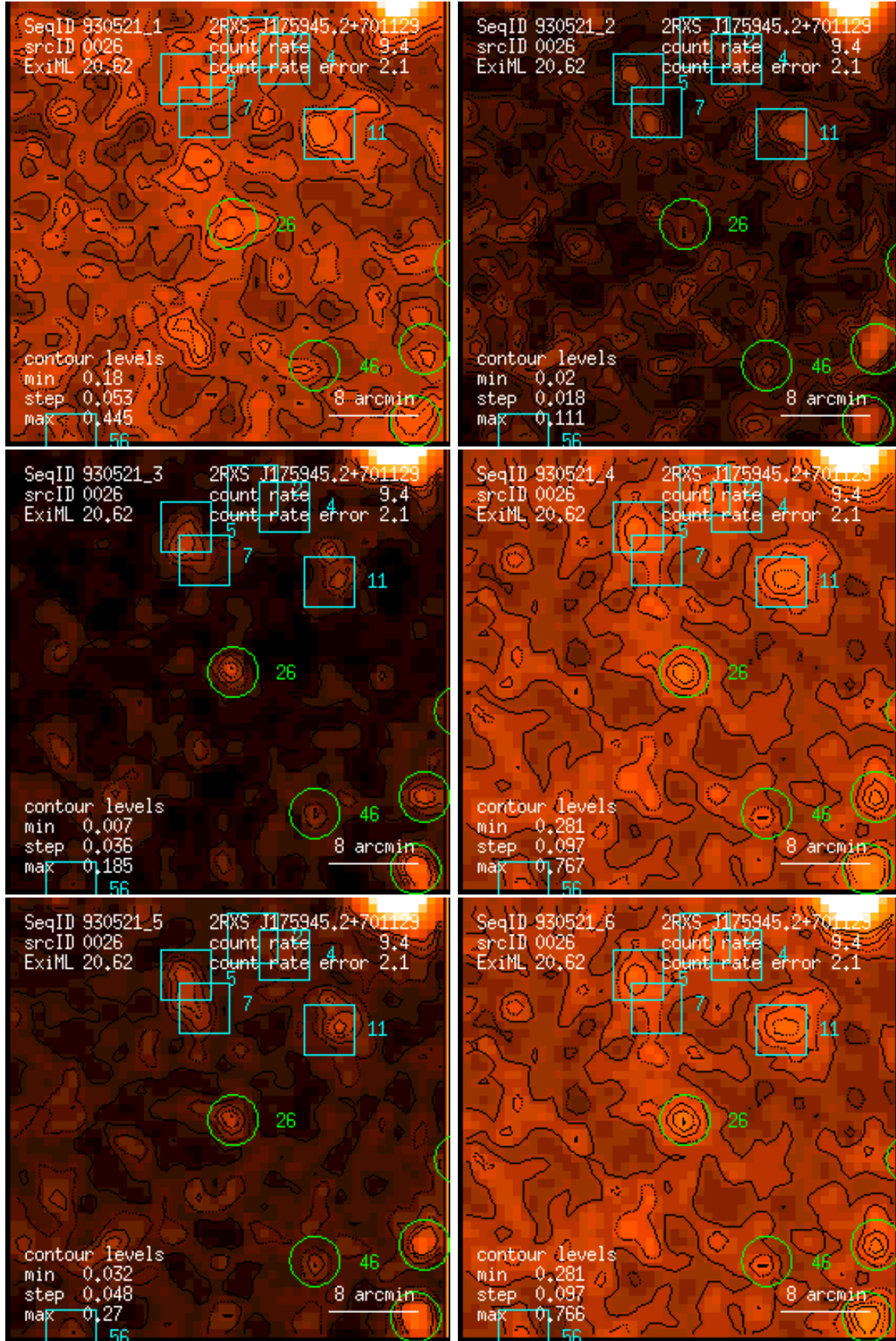
Figure 26: RASS 930521: detection 0026: band rate images, Gaussian filter: (1) PSPC channels 11 – 41, (2) 52 – 90, (3) 91 – 201, (4) 11 – 235, (5) 52 – 201, (6) 11 – 201. Broad band rates in counts/ks. Band rate contour levels in counts/ks/arcmin 2 .
