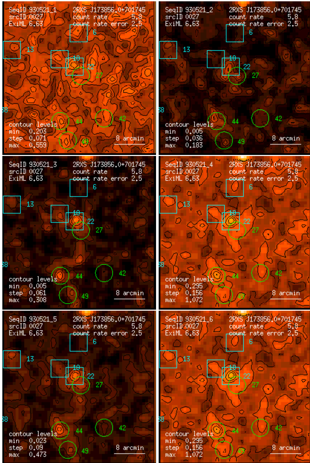
Figure 27: RASS 930521: detection 0027: band rate images, Gaussian filter: (1) PSPC channels 11 – 41, (2) 52 – 90, (3) 91 – 201, (4) 11 – 235, (5) 52 – 201, (6) 11 – 201. Broad band rates in counts/ks. Band rate contour levels in counts/ks/arcmin 2 .
