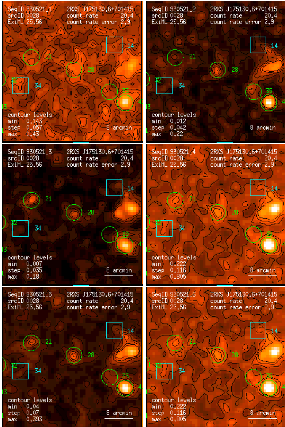
Figure 28: RASS 930521: detection 0028: band rate images, Gaussian filter: (1) PSPC channels 11 – 41, (2) 52 – 90, (3) 91 – 201, (4) 11 – 235, (5) 52 – 201, (6) 11 – 201. Broad band rates in counts/ks. Band rate contour levels in counts/ks/arcmin 2 .
