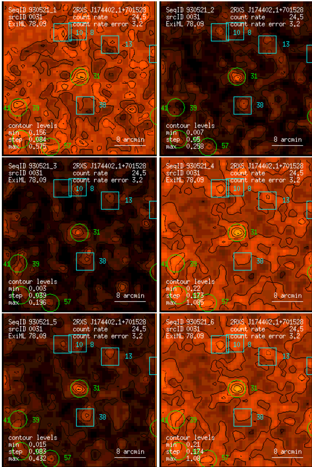
Figure 31: RASS 930521: detection 0031: band rate images, Gaussian filter: (1) PSPC channels 11 – 41, (2) 52 – 90, (3) 91 – 201, (4) 11 – 235, (5) 52 – 201, (6) 11 – 201. Broad band rates in counts/ks. Band rate contour levels in counts/ks/arcmin 2 .
