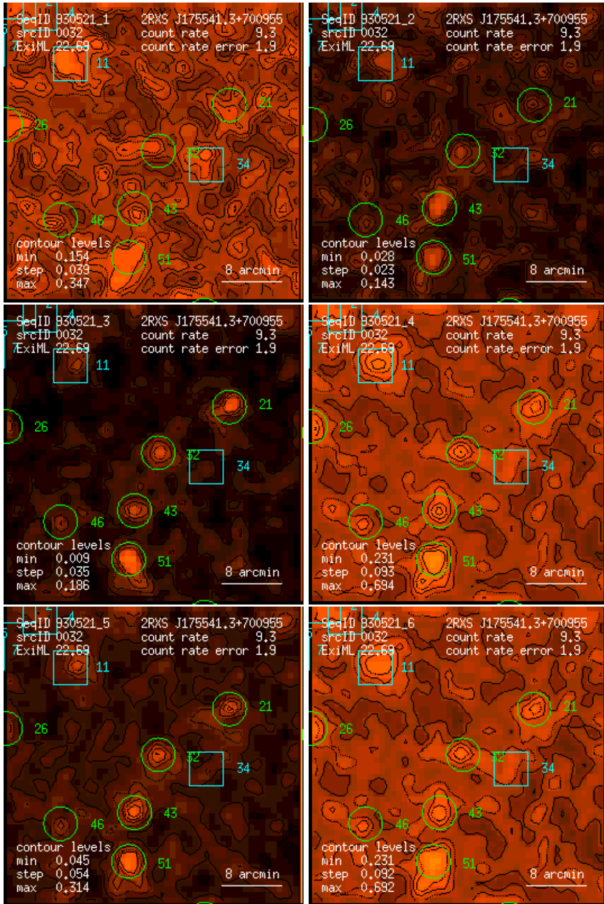
Figure 32: RASS 930521: detection 0032: band rate images, Gaussian filter: (1) PSPC channels 11 – 41, (2) 52 – 90, (3) 91 – 201, (4) 11 – 235, (5) 52 – 201, (6) 11 – 201. Broad band rates in counts/ks. Band rate contour levels in counts/ks/arcmin 2 .
