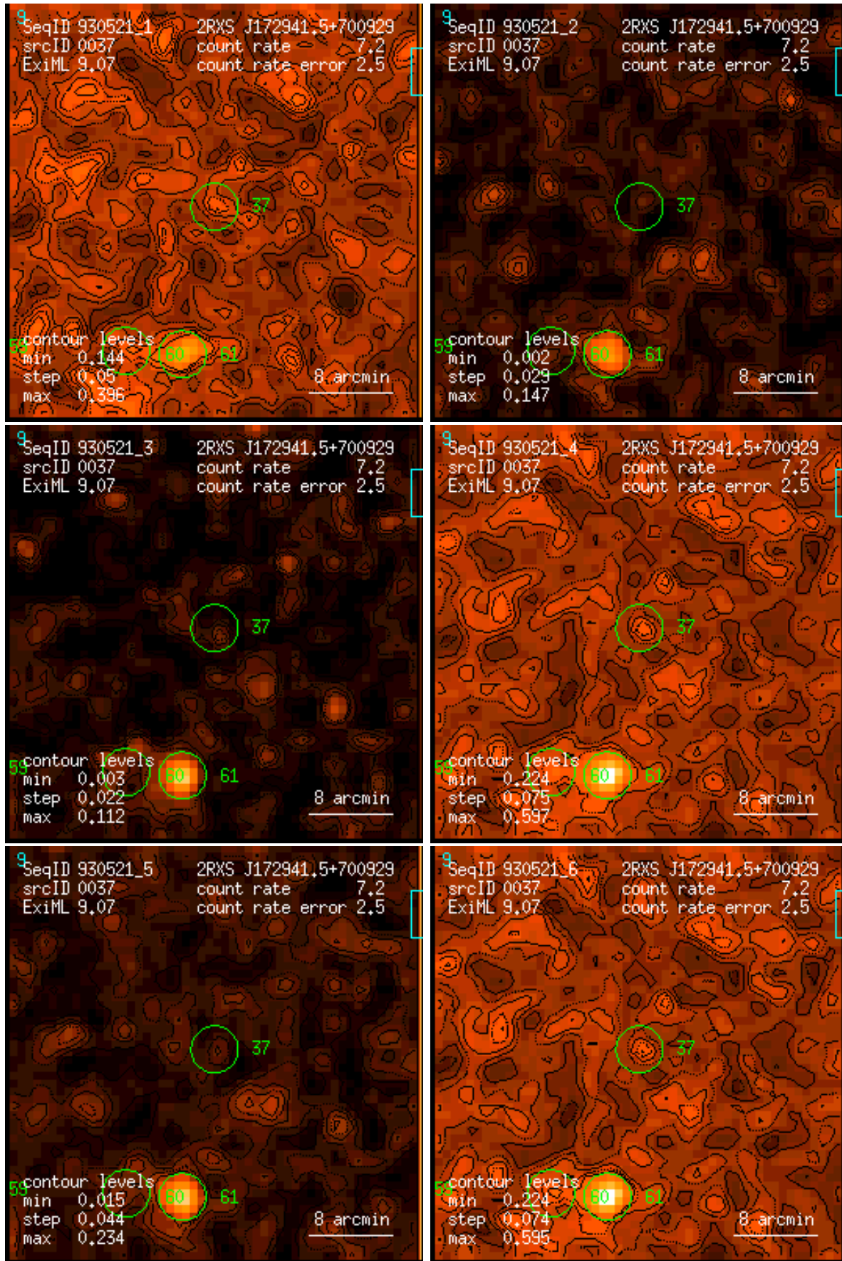
Figure 37: RASS 930521: detection 0037: band rate images, Gaussian filter: (1) PSPC channels 11 – 41, (2) 52 – 90, (3) 91 – 201, (4) 11 – 235, (5) 52 – 201, (6) 11 – 201. Broad band rates in counts/ks. Band rate contour levels in counts/ks/arcmin 2 .
