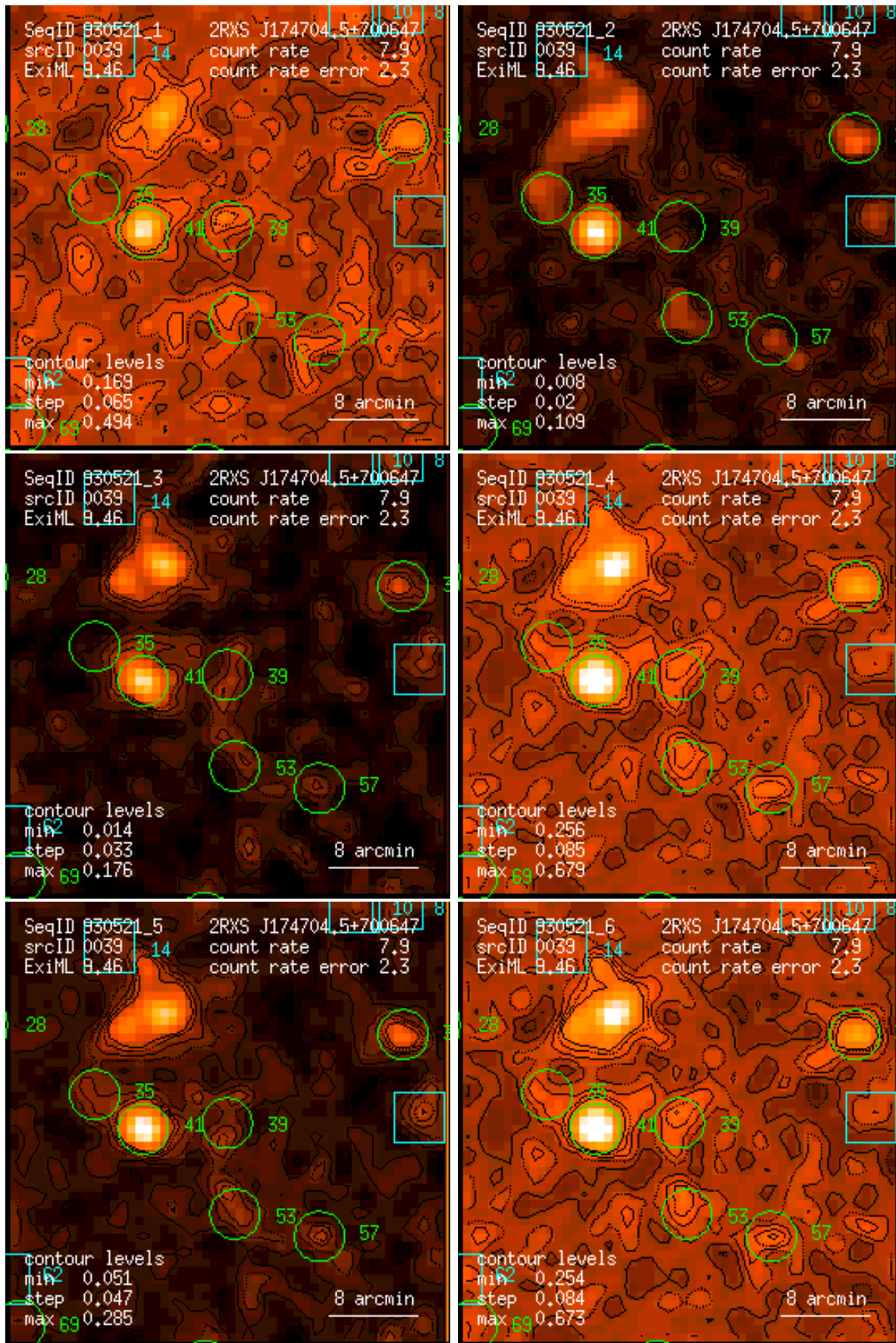
Figure 39: RASS 930521: detection 0039: band rate images, Gaussian filter: (1) PSPC channels 11 – 41, (2) 52 – 90, (3) 91 – 201, (4) 11 – 235, (5) 52 – 201, (6) 11 – 201. Broad band rates in counts/ks. Band rate contour levels in counts/ks/arcmin 2 .
