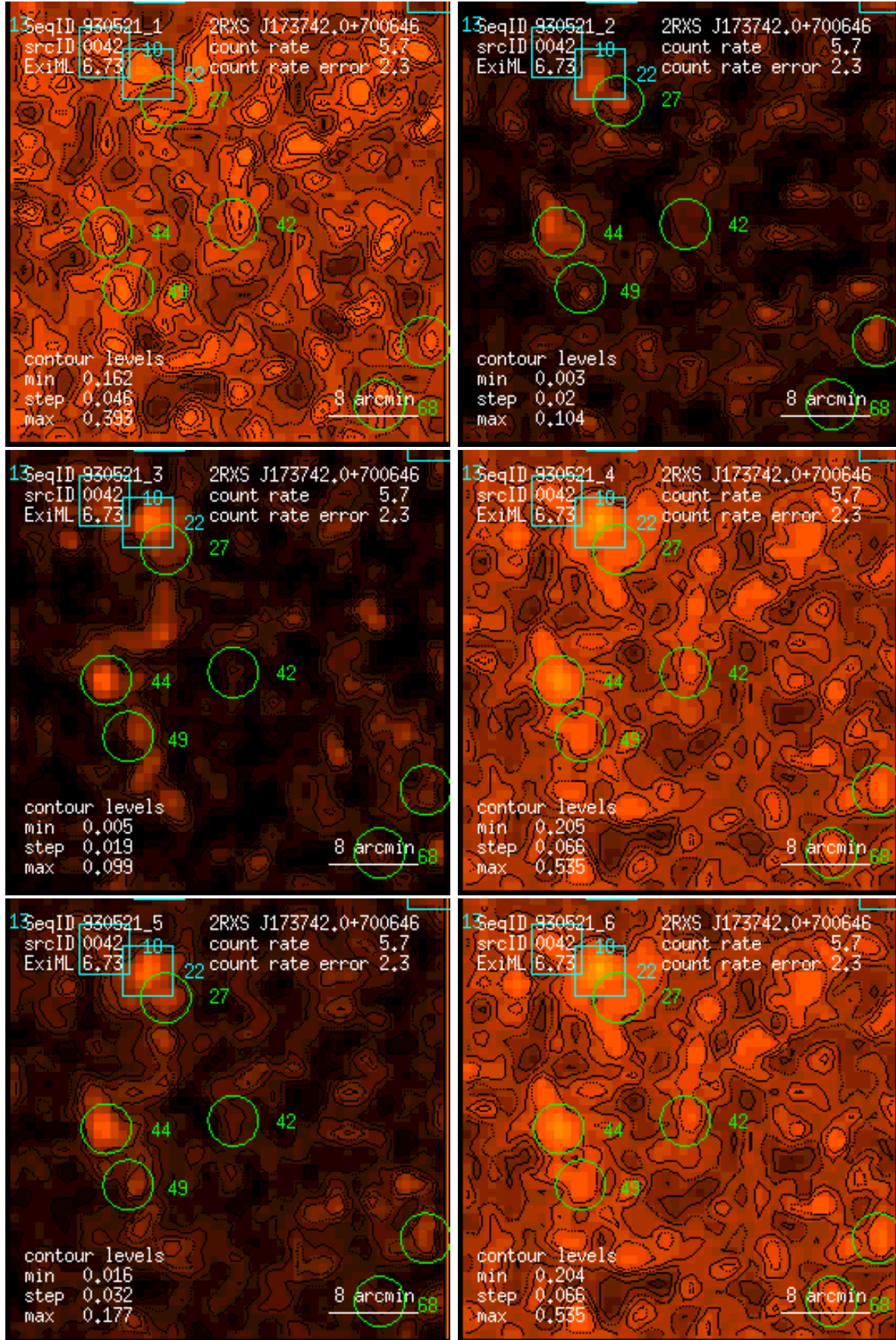
Figure 42: RASS 930521: detection 0042: band rate images, Gaussian filter: (1) PSPC channels 11 – 41, (2) 52 – 90, (3) 91 – 201, (4) 11 – 235, (5) 52 – 201, (6) 11 – 201. Broad band rates in counts/ks. Band rate contour levels in counts/ks/arcmin 2 .
