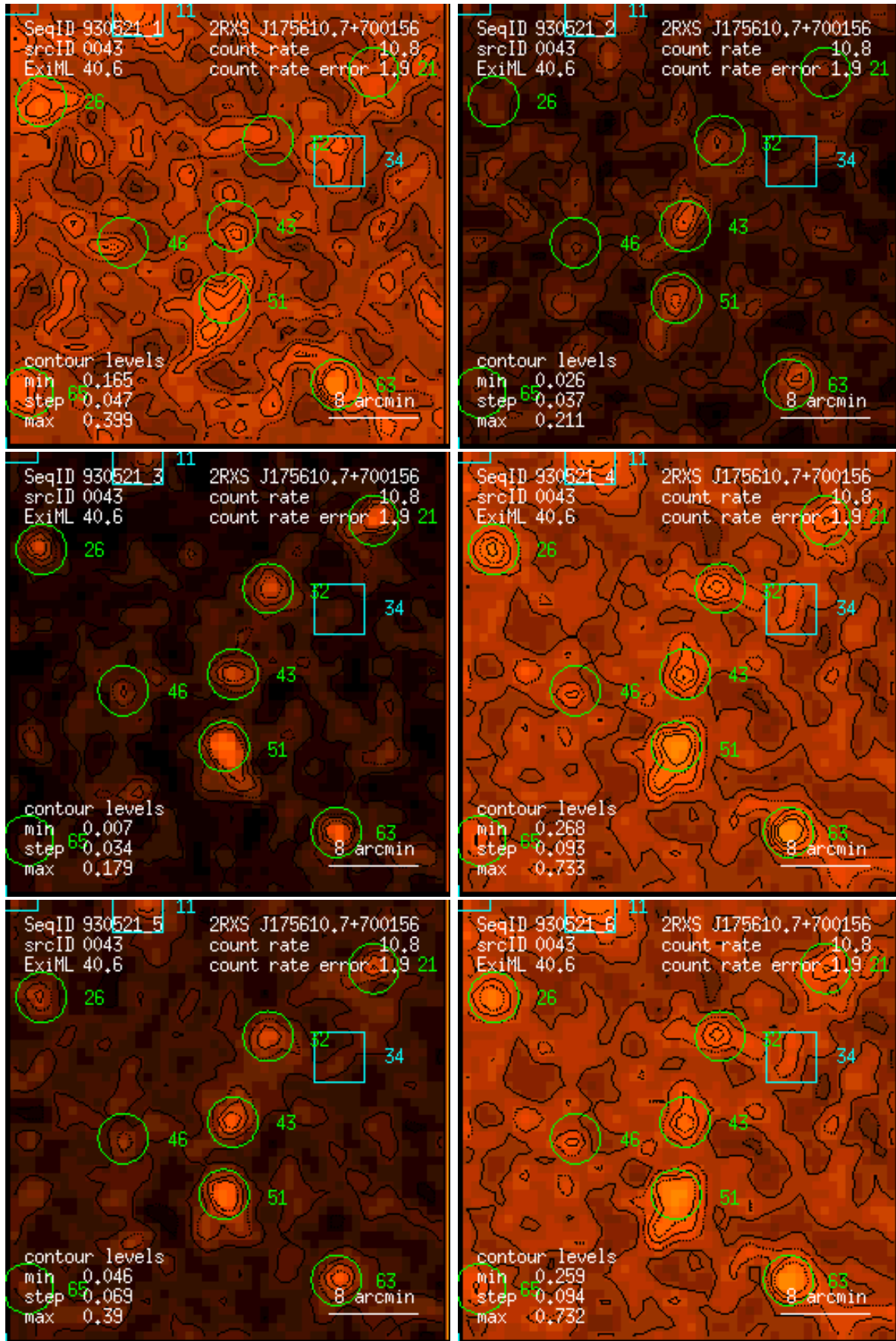
Figure 43: RASS 930521: detection 0043: band rate images, Gaussian filter: (1) PSPC channels 11 – 41, (2) 52 – 90, (3) 91 – 201, (4) 11 – 235, (5) 52 – 201, (6) 11 – 201. Broad band rates in counts/ks. Band rate contour levels in counts/ks/arcmin 2 .
