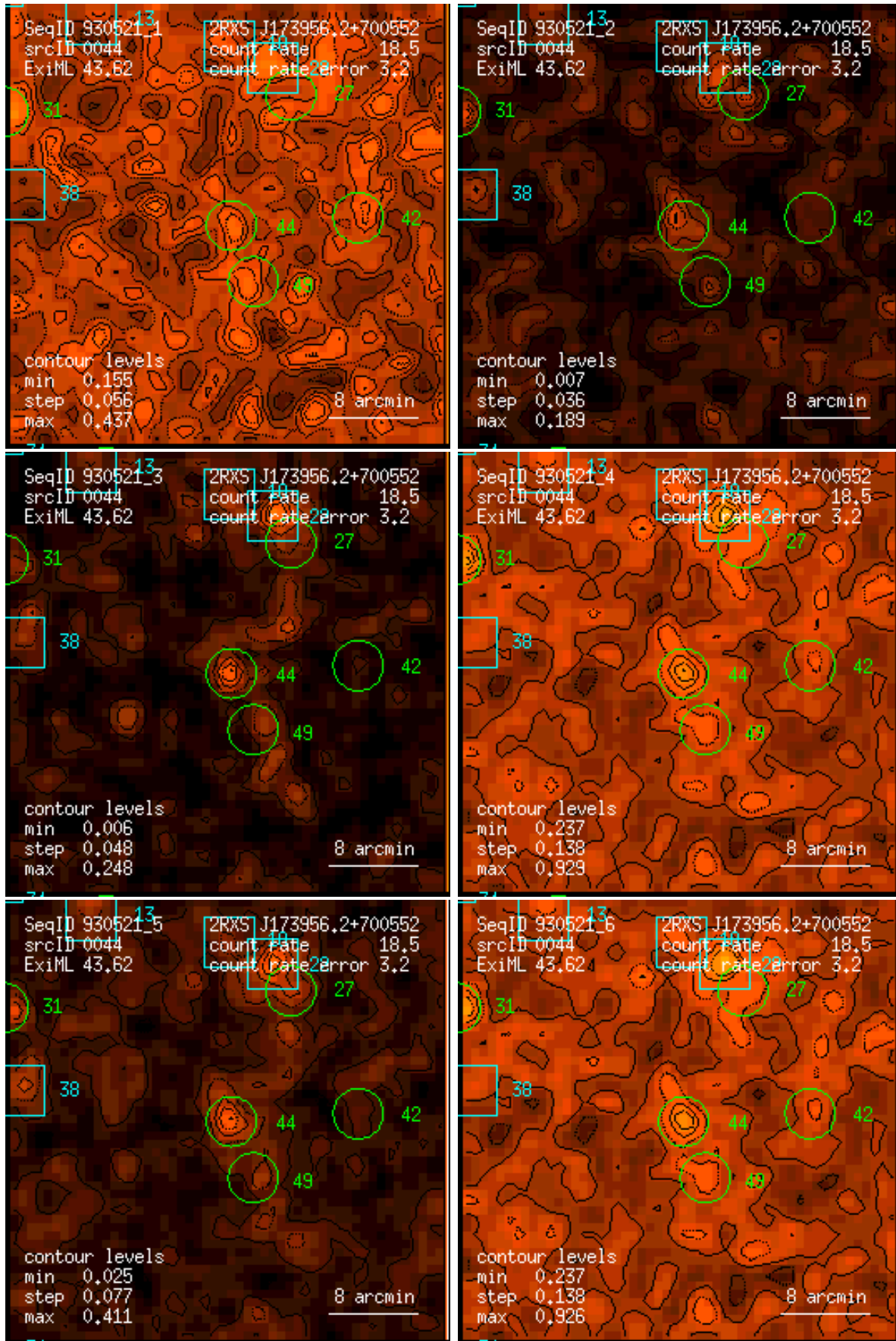
Figure 44: RASS 930521: detection 0044: band rate images, Gaussian filter: (1) PSPC channels 11 – 41, (2) 52 – 90, (3) 91 – 201, (4) 11 – 235, (5) 52 – 201, (6) 11 – 201. Broad band rates in counts/ks. Band rate contour levels in counts/ks/arcmin 2 .
