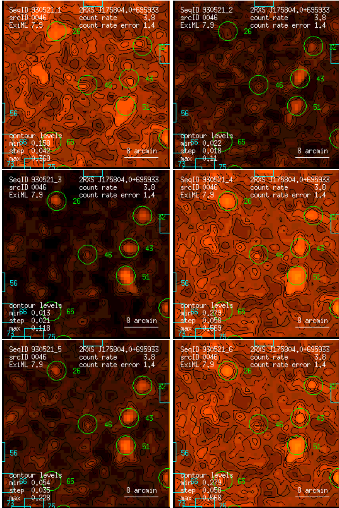
Figure 46: RASS 930521: detection 0046: band rate images, Gaussian filter: (1) PSPC channels 11 – 41, (2) 52 – 90, (3) 91 – 201, (4) 11 – 235, (5) 52 – 201, (6) 11 – 201. Broad band rates in counts/ks. Band rate contour levels in counts/ks/arcmin 2 .
