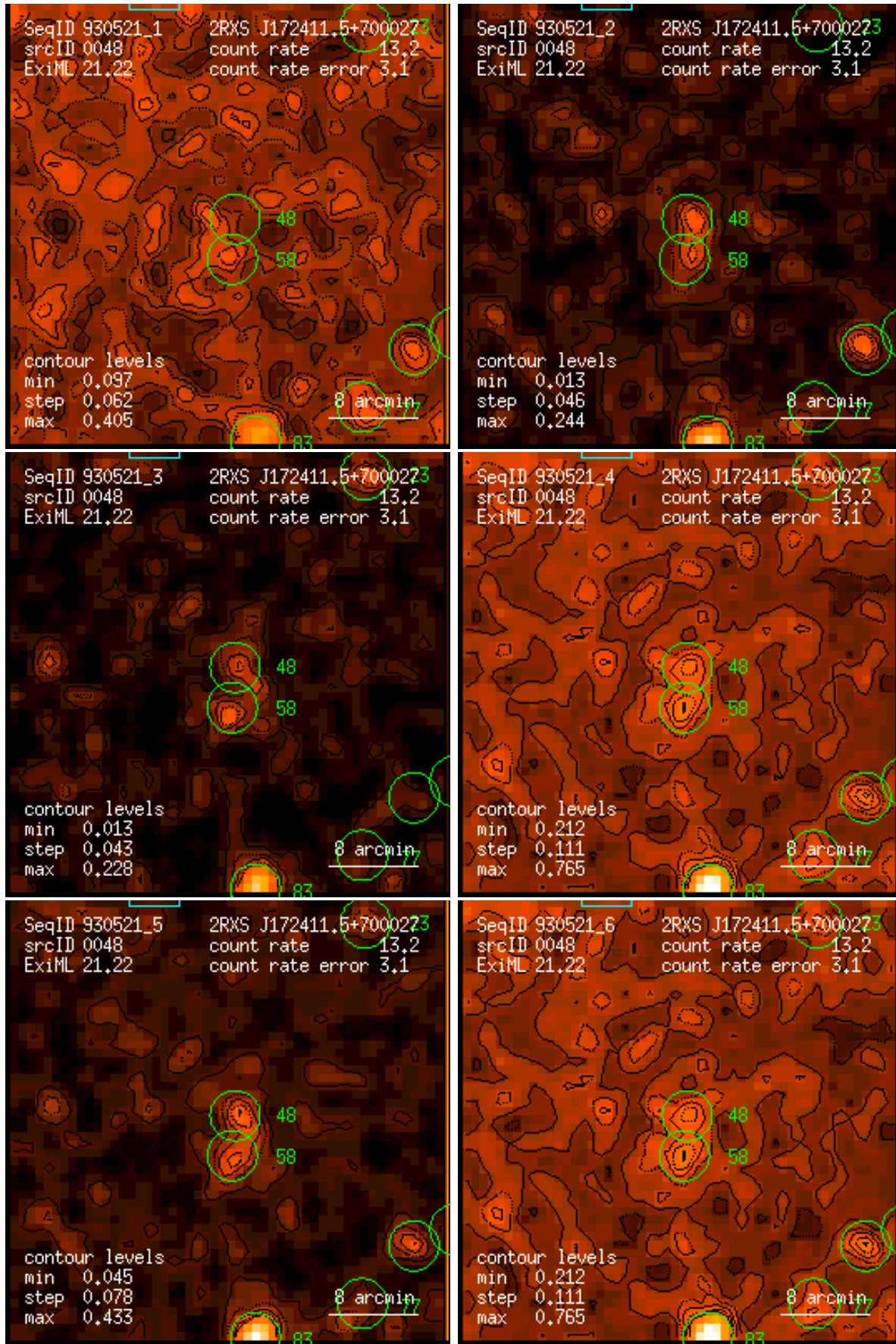
Figure 48: RASS 930521: detection 0048: band rate images, Gaussian filter: (1) PSPC channels 11 – 41, (2) 52 – 90, (3) 91 – 201, (4) 11 – 235, (5) 52 – 201, (6) 11 – 201. Broad band rates in counts/ks. Band rate contour levels in counts/ks/arcmin 2 .
