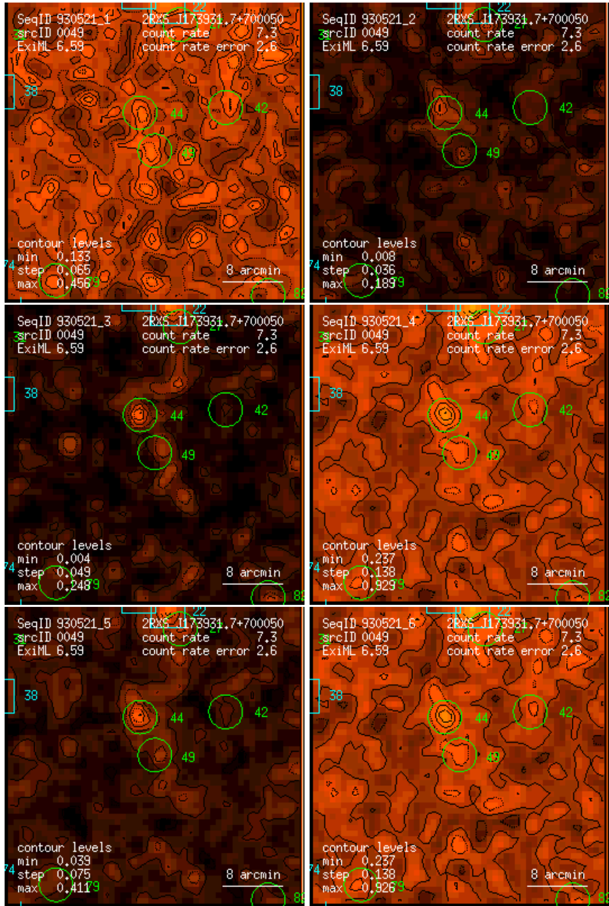
Figure 49: RASS 930521: detection 0049: band rate images, Gaussian filter: (1) PSPC channels 11 – 41, (2) 52 – 90, (3) 91 – 201, (4) 11 – 235, (5) 52 – 201, (6) 11 – 201. Broad band rates in counts/ks. Band rate contour levels in counts/ks/arcmin 2 .
