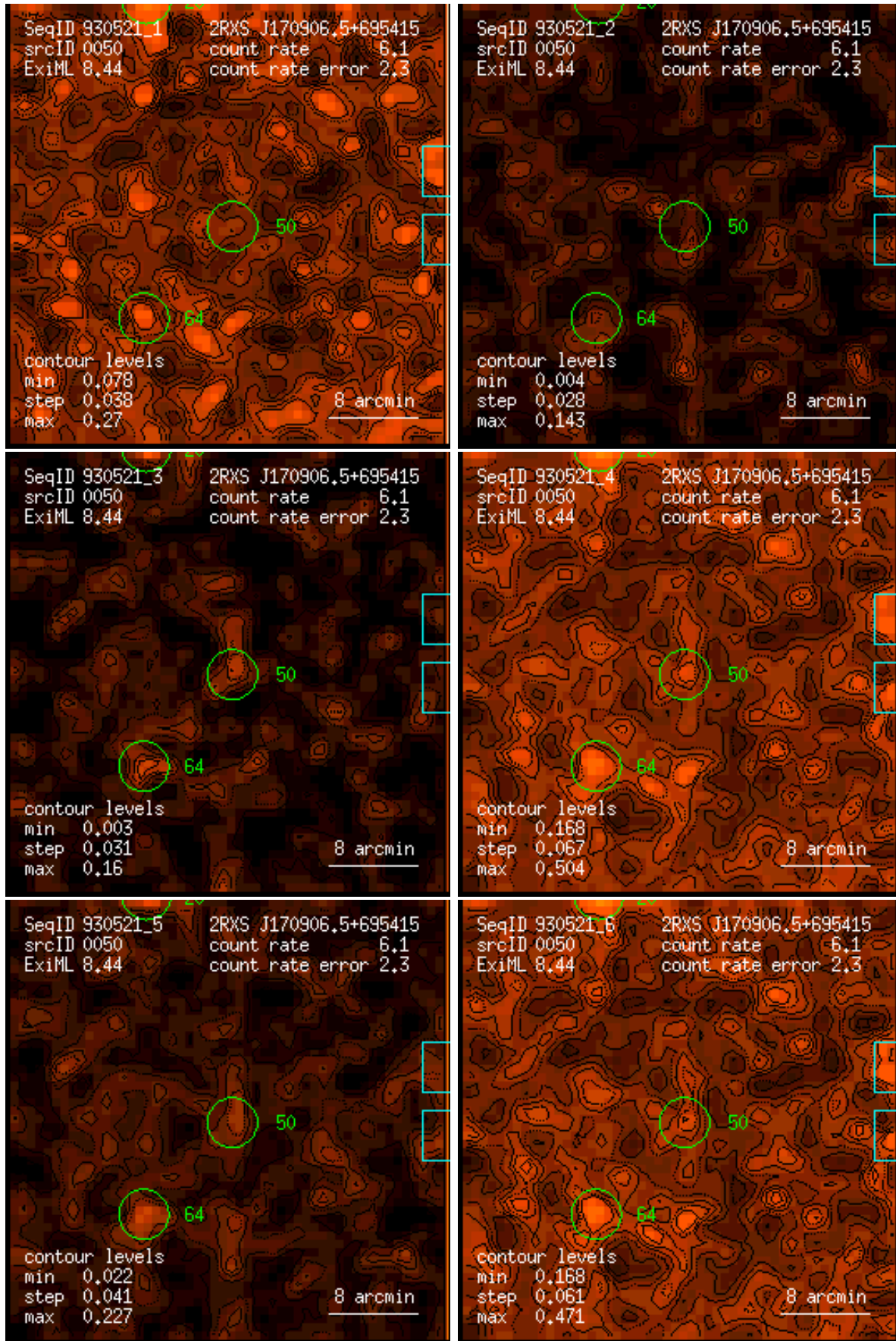
Figure 50: RASS 930521: detection 0050: band rate images, Gaussian filter: (1) PSPC channels 11 – 41, (2) 52 – 90, (3) 91 – 201, (4) 11 – 235, (5) 52 – 201, (6) 11 – 201. Broad band rates in counts/ks. Band rate contour levels in counts/ks/arcmin 2 .
