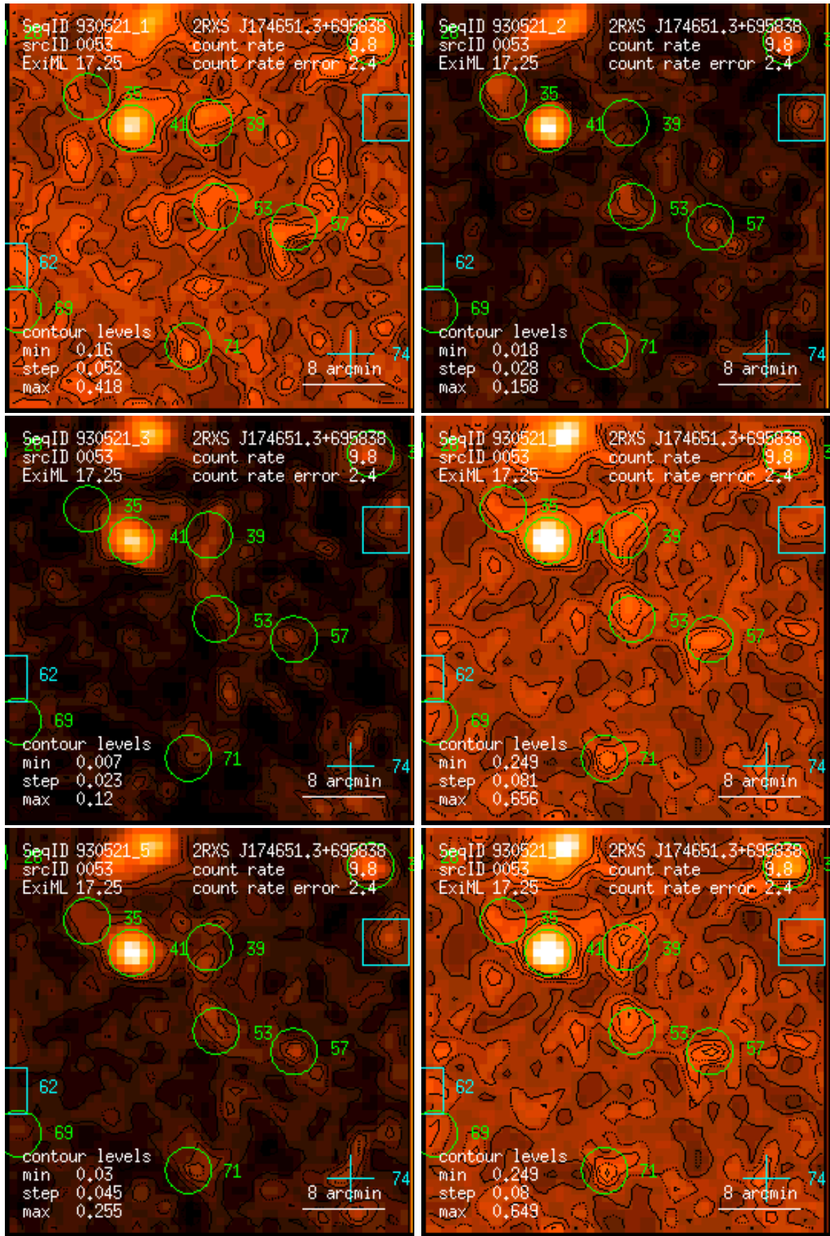
Figure 53: RASS 930521: detection 0053: band rate images, Gaussian filter: (1) PSPC channels 11 – 41, (2) 52 – 90, (3) 91 – 201, (4) 11 – 235, (5) 52 – 201, (6) 11 – 201. Broad band rates in counts/ks. Band rate contour levels in counts/ks/arcmin 2 .
