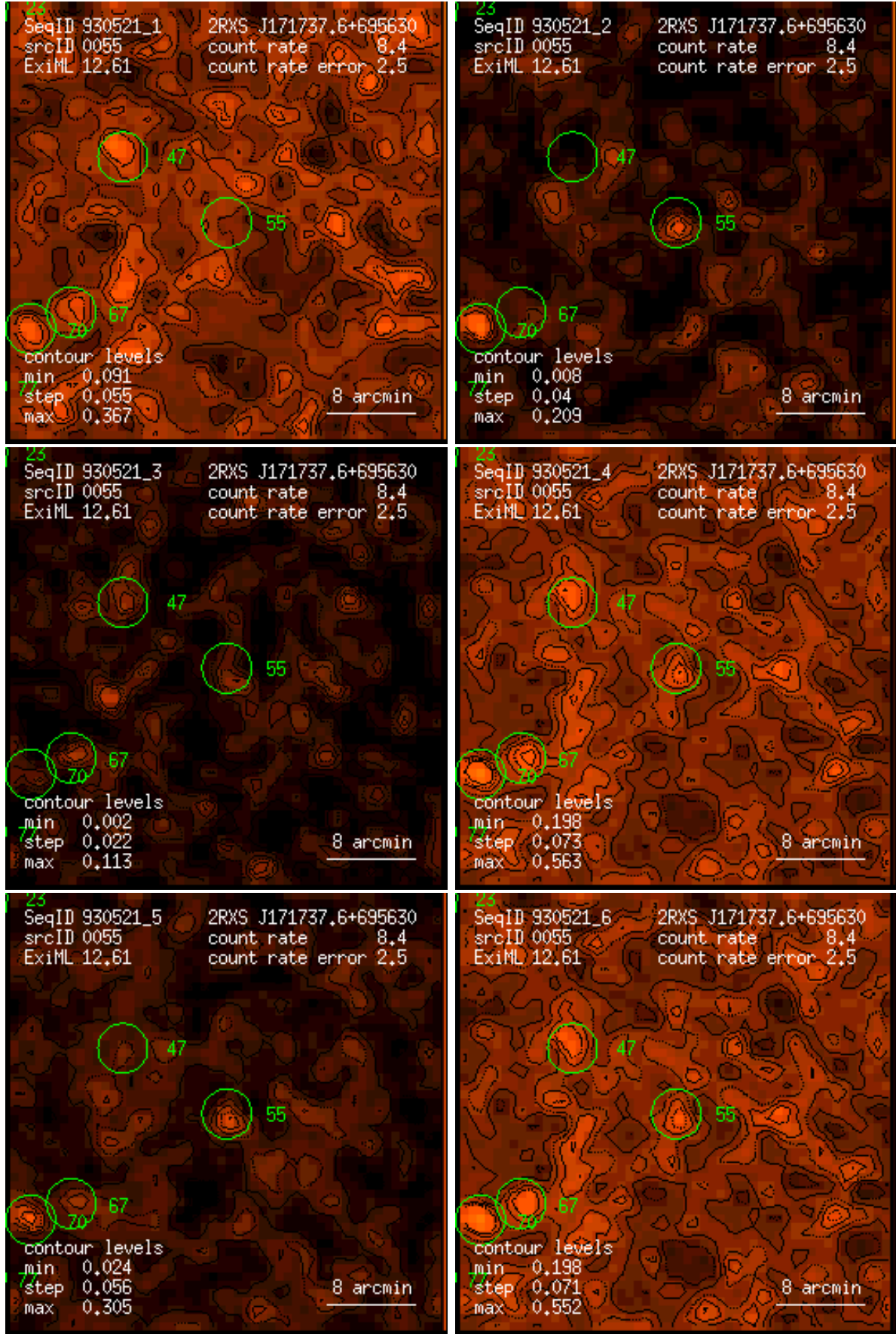
Figure 55: RASS 930521: detection 0055: band rate images, Gaussian filter: (1) PSPC channels 11 – 41, (2) 52 – 90, (3) 91 – 201, (4) 11 – 235, (5) 52 – 201, (6) 11 – 201. Broad band rates in counts/ks. Band rate contour levels in counts/ks/arcmin 2 .
