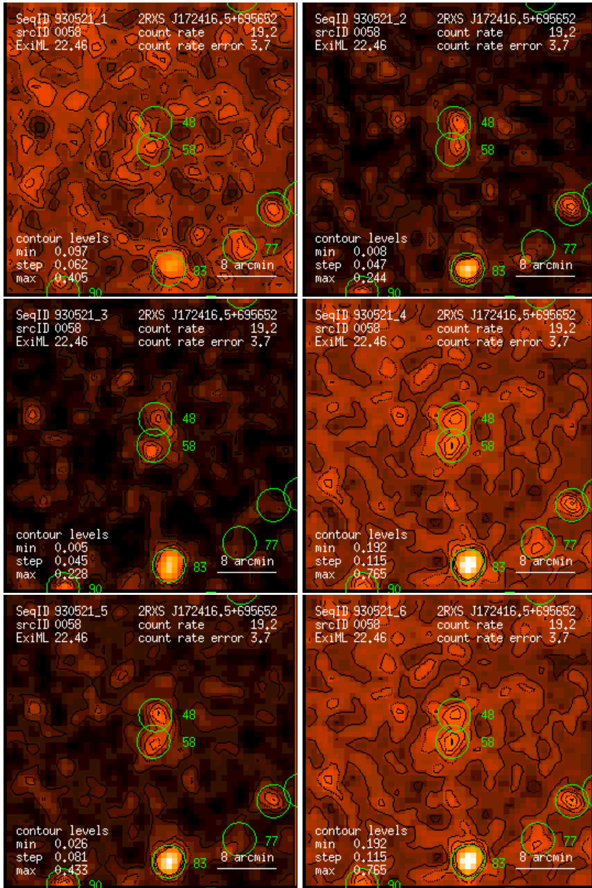
Figure 58: RASS 930521: detection 0058: band rate images, Gaussian filter: (1) PSPC channels 11 – 41, (2) 52 – 90, (3) 91 – 201, (4) 11 – 235, (5) 52 – 201, (6) 11 – 201. Broad band rates in counts/ks. Band rate contour levels in counts/ks/arcmin 2 .
