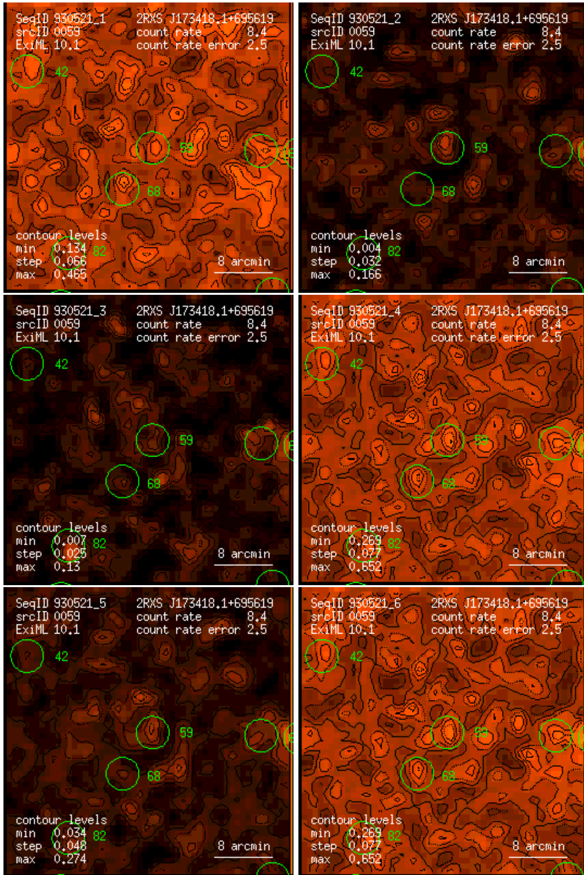
Figure 59: RASS 930521: detection 0059: band rate images, Gaussian filter: (1) PSPC channels 11 – 41, (2) 52 – 90, (3) 91 – 201, (4) 11 – 235, (5) 52 – 201, (6) 11 – 201. Broad band rates in counts/ks. Band rate contour levels in counts/ks/arcmin 2 .
