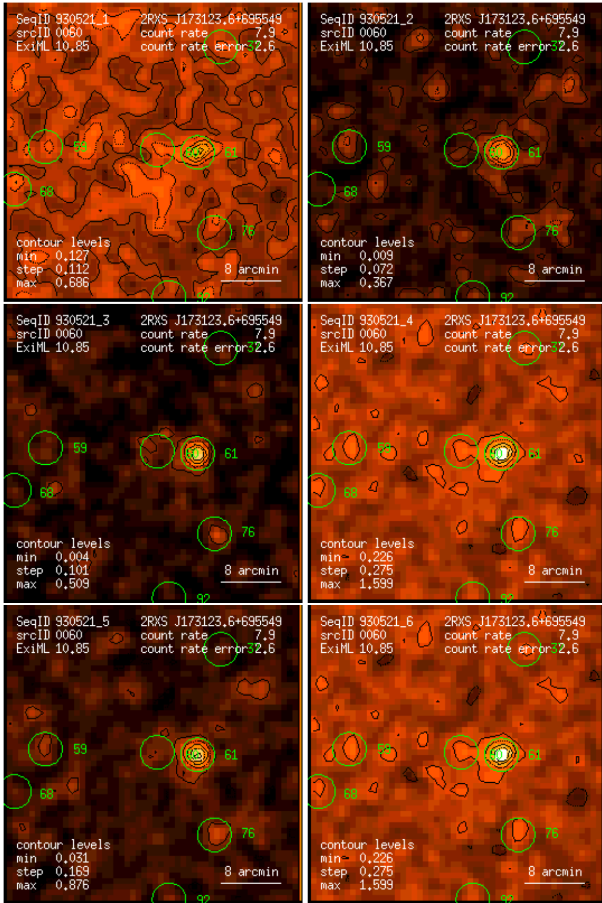
Figure 60: RASS 930521: detection 0060: band rate images, Gaussian filter: (1) PSPC channels 11 – 41, (2) 52 – 90, (3) 91 – 201, (4) 11 – 235, (5) 52 – 201, (6) 11 – 201. Broad band rates in counts/ks. Band rate contour levels in counts/ks/arcmin 2 .
