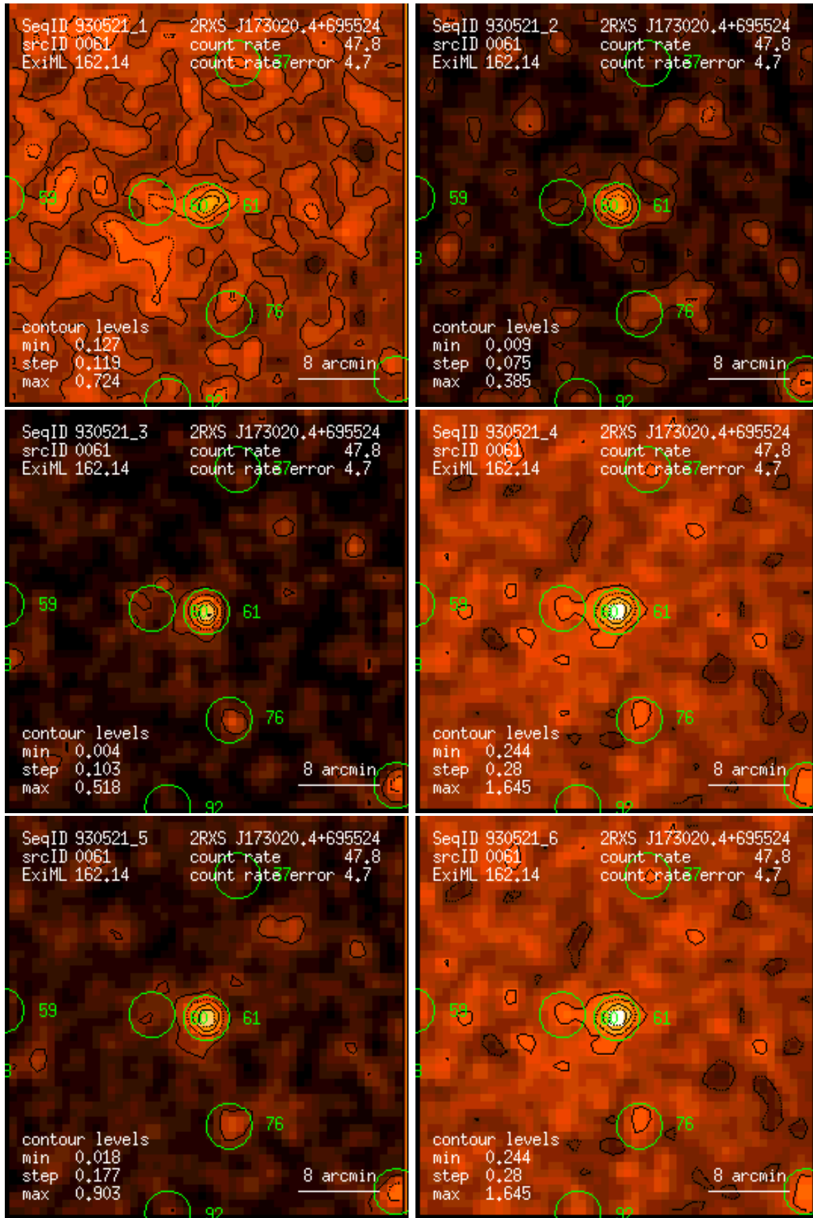
Figure 61: RASS 930521: detection 0061: band rate images, Gaussian filter: (1) PSPC channels 11 – 41, (2) 52 – 90, (3) 91 – 201, (4) 11 – 235, (5) 52 – 201, (6) 11 – 201. Broad band rates in counts/ks. Band rate contour levels in counts/ks/arcmin 2 .
