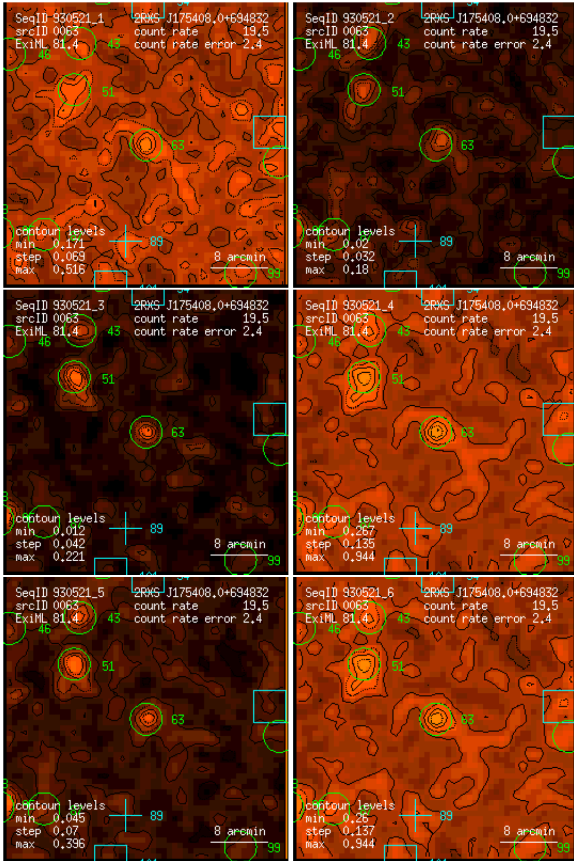
Figure 63: RASS 930521: detection 0063: band rate images, Gaussian filter: (1) PSPC channels 11 – 41, (2) 52 – 90, (3) 91 – 201, (4) 11 – 235, (5) 52 – 201, (6) 11 – 201. Broad band rates in counts/ks. Band rate contour levels in counts/ks/arcmin 2 .
