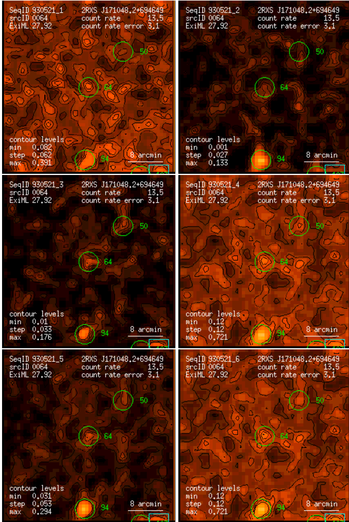
Figure 64: RASS 930521: detection 0064: band rate images, Gaussian filter: (1) PSPC channels 11 – 41, (2) 52 – 90, (3) 91 – 201, (4) 11 – 235, (5) 52 – 201, (6) 11 – 201. Broad band rates in counts/ks. Band rate contour levels in counts/ks/arcmin 2 .
