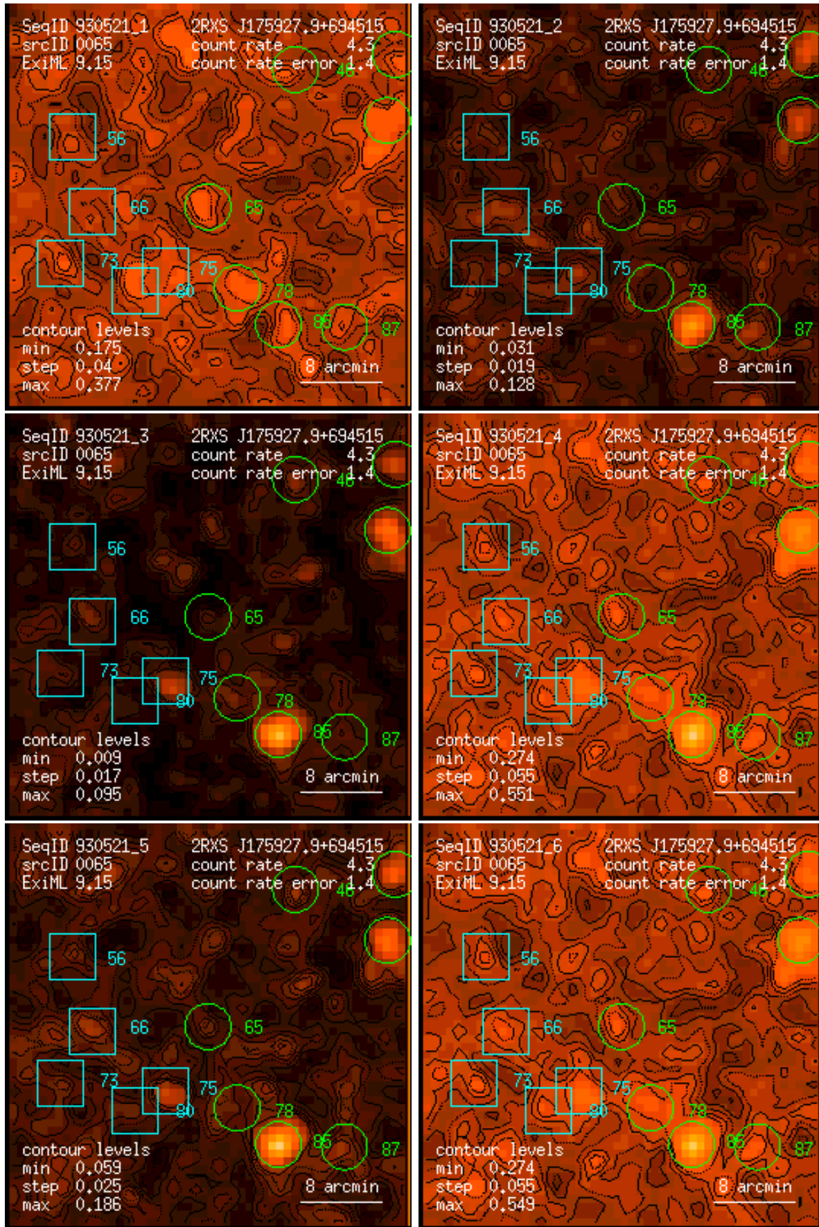
Figure 65: RASS 930521: detection 0065: band rate images, Gaussian filter: (1) PSPC channels 11 – 41, (2) 52 – 90, (3) 91 – 201, (4) 11 – 235, (5) 52 – 201, (6) 11 – 201. Broad band rates in counts/ks. Band rate contour levels in counts/ks/arcmin 2 .
