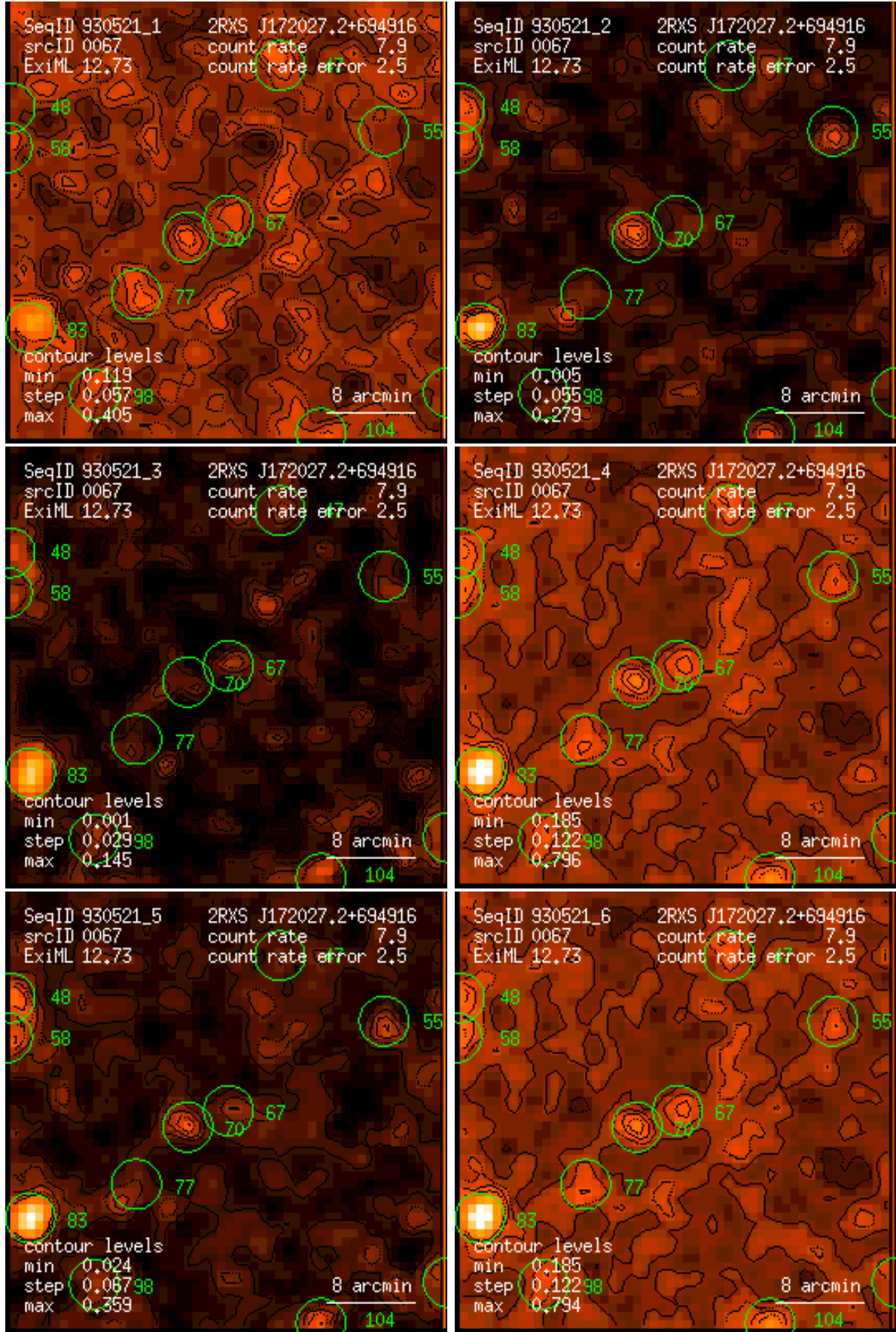
Figure 67: RASS 930521: detection 0067: band rate images, Gaussian filter: (1) PSPC channels 11 – 41, (2) 52 – 90, (3) 91 – 201, (4) 11 – 235, (5) 52 – 201, (6) 11 – 201. Broad band rates in counts/ks. Band rate contour levels in counts/ks/arcmin 2 .
