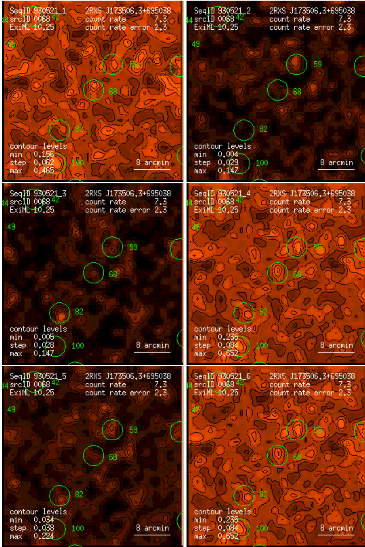
Figure 68: RASS 930521: detection 0068: band rate images, Gaussian filter: (1) PSPC channels 11 – 41, (2) 52 – 90, (3) 91 – 201, (4) 11 – 235, (5) 52 – 201, (6) 11 – 201. Broad band rates in counts/ks. Band rate contour levels in counts/ks/arcmin 2 .
