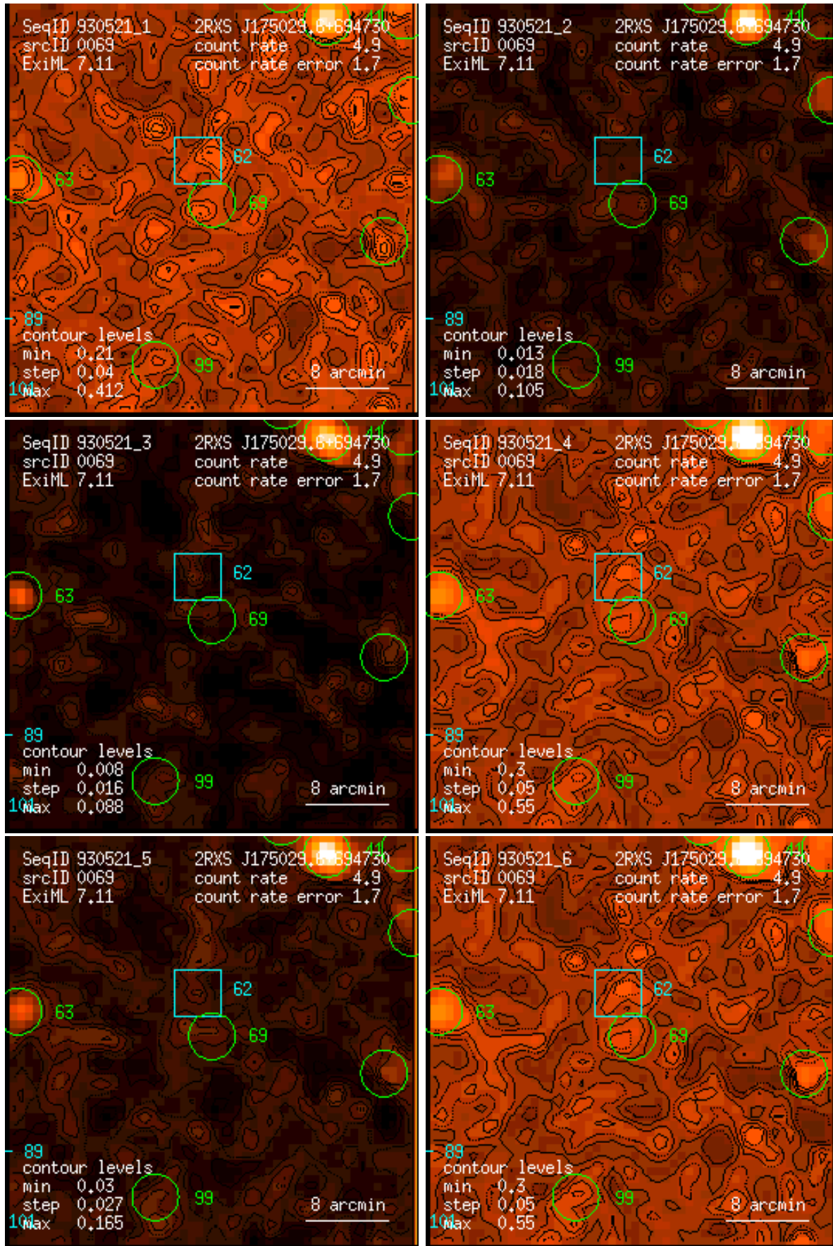
Figure 69: RASS 930521: detection 0069: band rate images, Gaussian filter: (1) PSPC channels 11 – 41, (2) 52 – 90, (3) 91 – 201, (4) 11 – 235, (5) 52 – 201, (6) 11 – 201. Broad band rates in counts/ks. Band rate contour levels in counts/ks/arcmin 2 .
