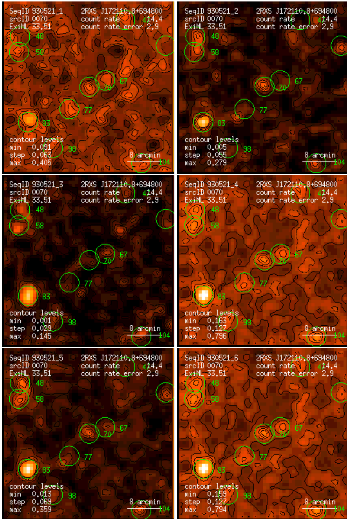
Figure 70: RASS 930521: detection 0070: band rate images, Gaussian filter: (1) PSPC channels 11 – 41, (2) 52 – 90, (3) 91 – 201, (4) 11 – 235, (5) 52 – 201, (6) 11 – 201. Broad band rates in counts/ks. Band rate contour levels in counts/ks/arcmin 2 .
