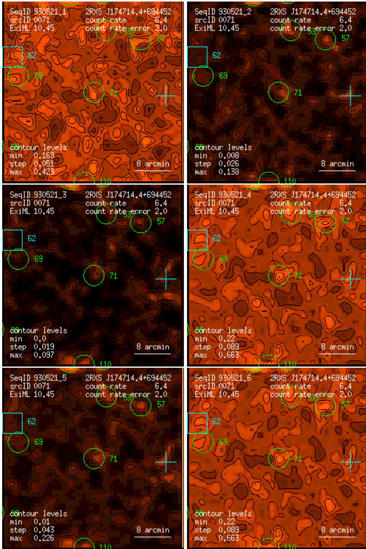
Figure 71: RASS 930521: detection 0071: band rate images, Gaussian filter: (1) PSPC channels 11 – 41, (2) 52 – 90, (3) 91 – 201, (4) 11 – 235, (5) 52 – 201, (6) 11 – 201. Broad band rates in counts/ks. Band rate contour levels in counts/ks/arcmin 2 .
