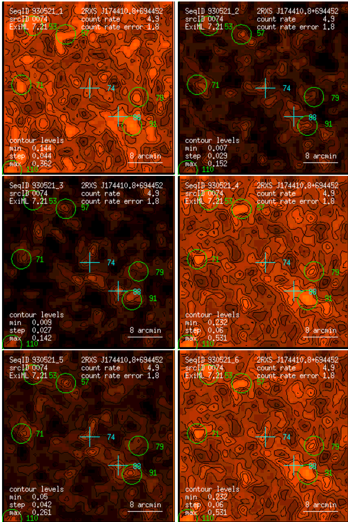
Figure 74: RASS 930521: detection 0074: band rate images, Gaussian filter: (1) PSPC channels 11 – 41, (2) 52 – 90, (3) 91 – 201, (4) 11 – 235, (5) 52 – 201, (6) 11 – 201. Broad band rates in counts/ks. Band rate contour levels in counts/ks/arcmin 2 .
