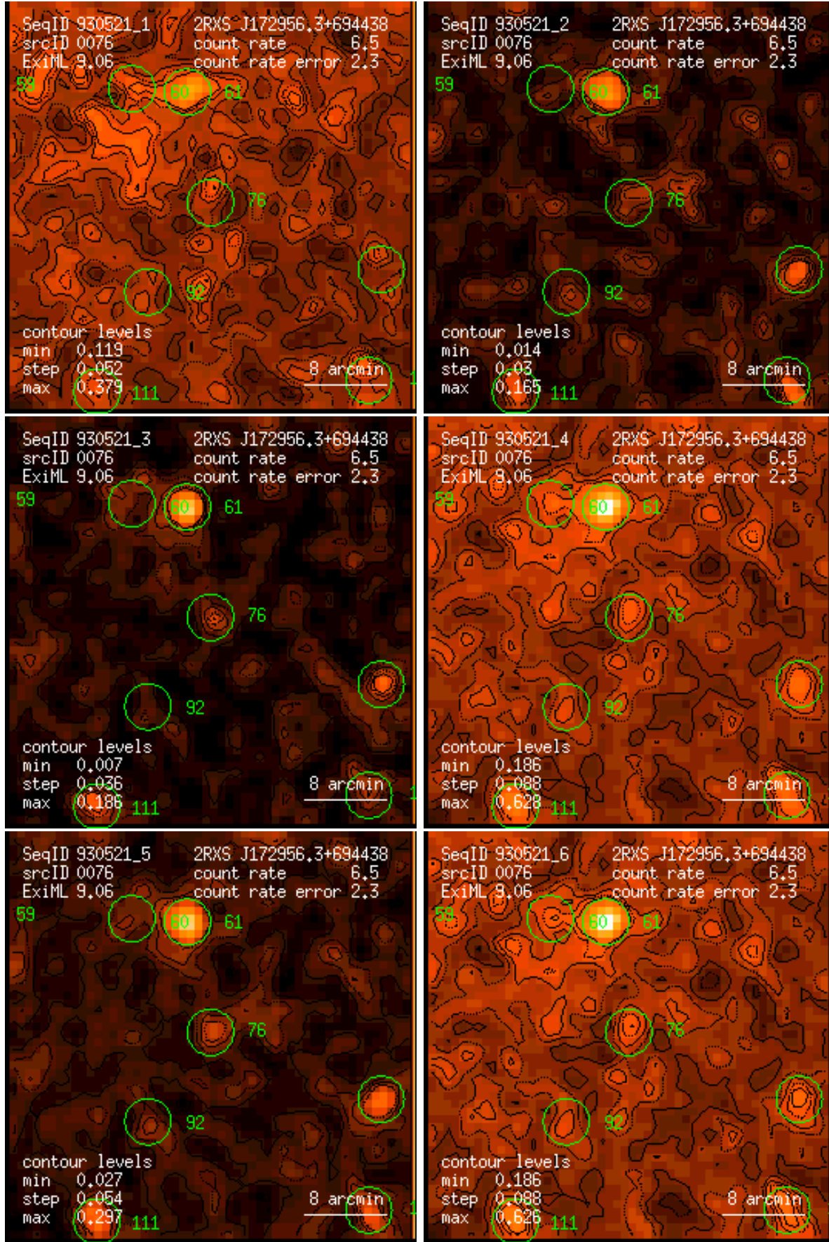
Figure 76: RASS 930521: detection 0076: band rate images, Gaussian filter: (1) PSPC channels 11 – 41, (2) 52 – 90, (3) 91 – 201, (4) 11 – 235, (5) 52 – 201, (6) 11 – 201. Broad band rates in counts/ks. Band rate contour levels in counts/ks/arcmin 2 .
