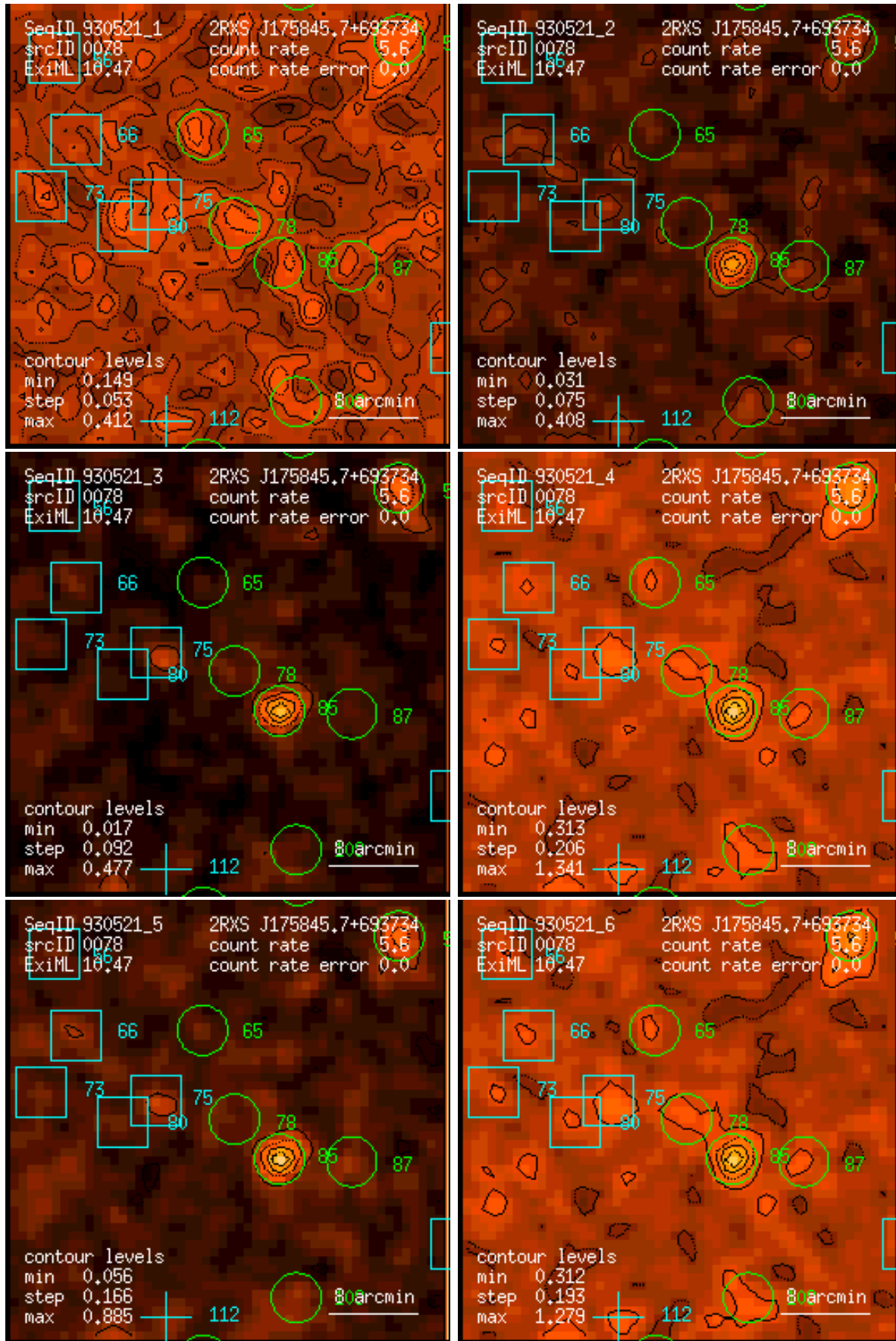
Figure 78: RASS 930521: detection 0078: band rate images, Gaussian filter: (1) PSPC channels 11 – 41, (2) 52 – 90, (3) 91 – 201, (4) 11 – 235, (5) 52 – 201, (6) 11 – 201. Broad band rates in counts/ks. Band rate contour levels in counts/ks/arcmin 2 .
