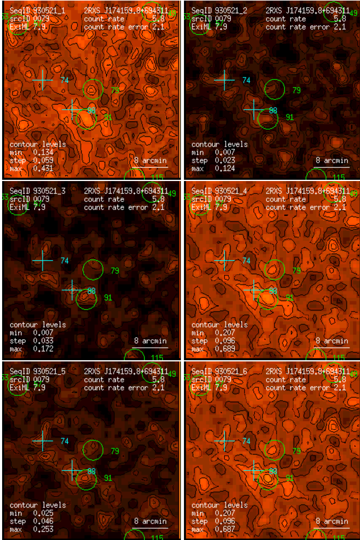
Figure 79: RASS 930521: detection 0079: band rate images, Gaussian filter: (1) PSPC channels 11 – 41, (2) 52 – 90, (3) 91 – 201, (4) 11 – 235, (5) 52 – 201, (6) 11 – 201. Broad band rates in counts/ks. Band rate contour levels in counts/ks/arcmin 2 .
