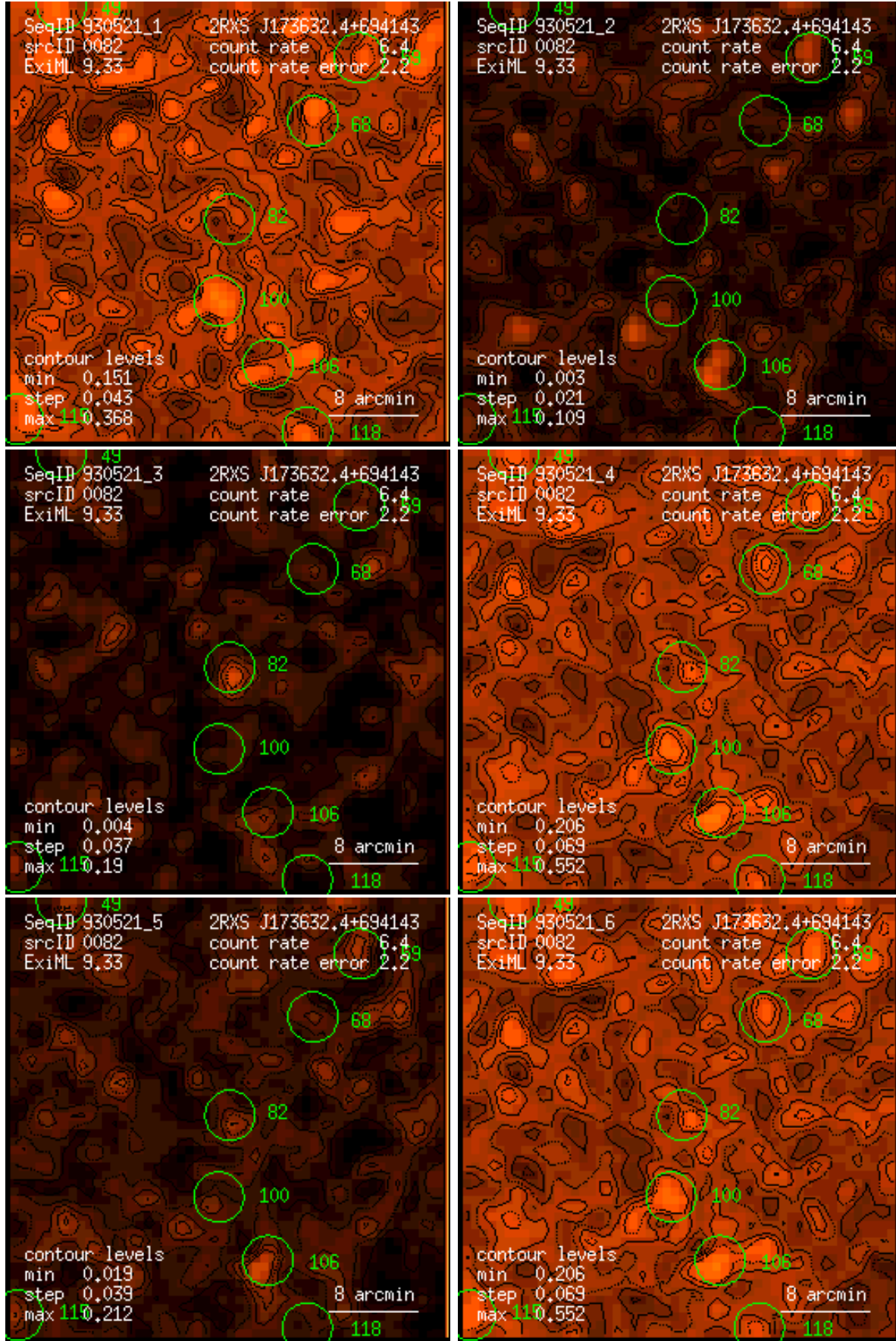
Figure 82: RASS 930521: detection 0082: band rate images, Gaussian filter: (1) PSPC channels 11 – 41, (2) 52 – 90, (3) 91 – 201, (4) 11 – 235, (5) 52 – 201, (6) 11 – 201. Broad band rates in counts/ks. Band rate contour levels in counts/ks/arcmin 2 .
