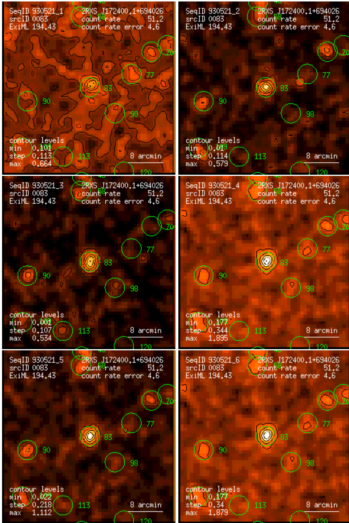
Figure 83: RASS 930521: detection 0083: band rate images, Gaussian filter: (1) PSPC channels 11 – 41, (2) 52 – 90, (3) 91 – 201, (4) 11 – 235, (5) 52 – 201, (6) 11 – 201. Broad band rates in counts/ks. Band rate contour levels in counts/ks/arcmin 2 .
