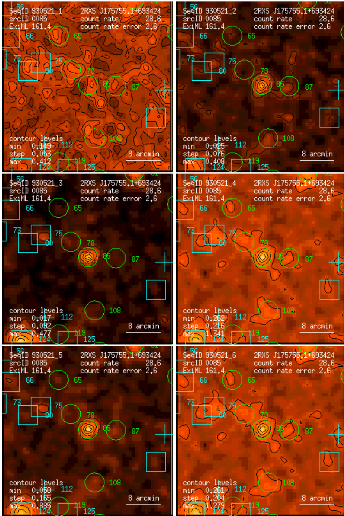
Figure 85: RASS 930521: detection 0085: band rate images, Gaussian filter: (1) PSPC channels 11 – 41, (2) 52 – 90, (3) 91 – 201, (4) 11 – 235, (5) 52 – 201, (6) 11 – 201. Broad band rates in counts/ks. Band rate contour levels in counts/ks/arcmin 2 .
