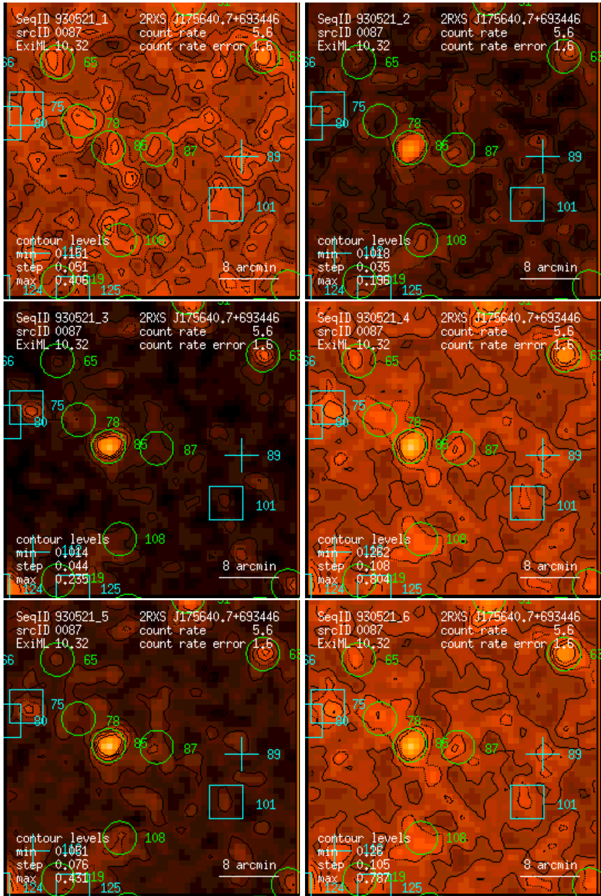
Figure 87: RASS 930521: detection 0087: band rate images, Gaussian filter: (1) PSPC channels 11 – 41, (2) 52 – 90, (3) 91 – 201, (4) 11 – 235, (5) 52 – 201, (6) 11 – 201. Broad band rates in counts/ks. Band rate contour levels in counts/ks/arcmin 2 .
