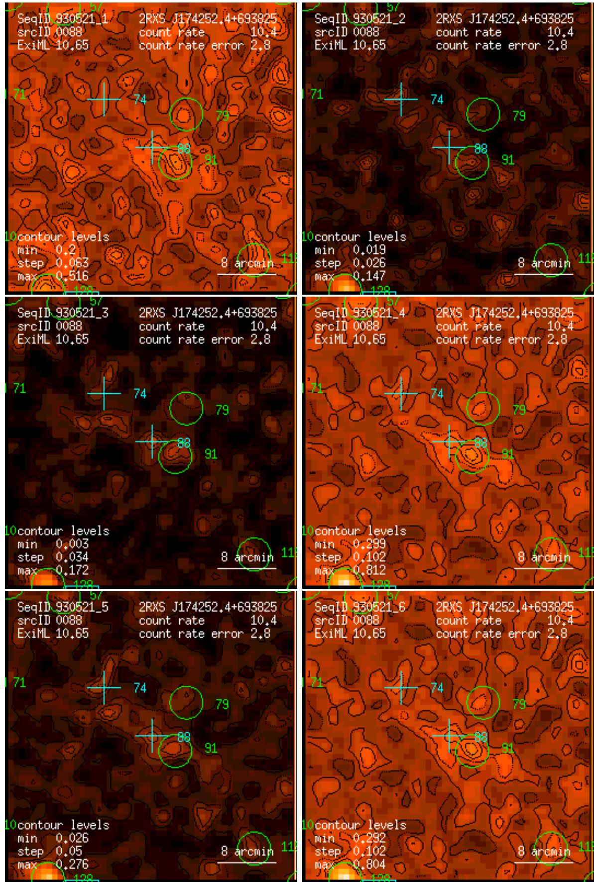
Figure 88: RASS 930521: detection 0088: band rate images, Gaussian filter: (1) PSPC channels 11 – 41, (2) 52 – 90, (3) 91 – 201, (4) 11 – 235, (5) 52 – 201, (6) 11 – 201. Broad band rates in counts/ks. Band rate contour levels in counts/ks/arcmin 2 .
