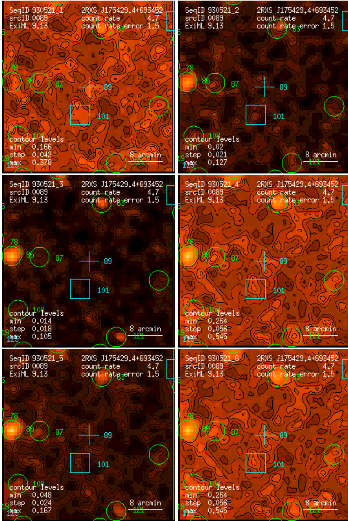
Figure 89: RASS 930521: detection 0089: band rate images, Gaussian filter: (1) PSPC channels 11 – 41, (2) 52 – 90, (3) 91 – 201, (4) 11 – 235, (5) 52 – 201, (6) 11 – 201. Broad band rates in counts/ks. Band rate contour levels in counts/ks/arcmin 2 .
