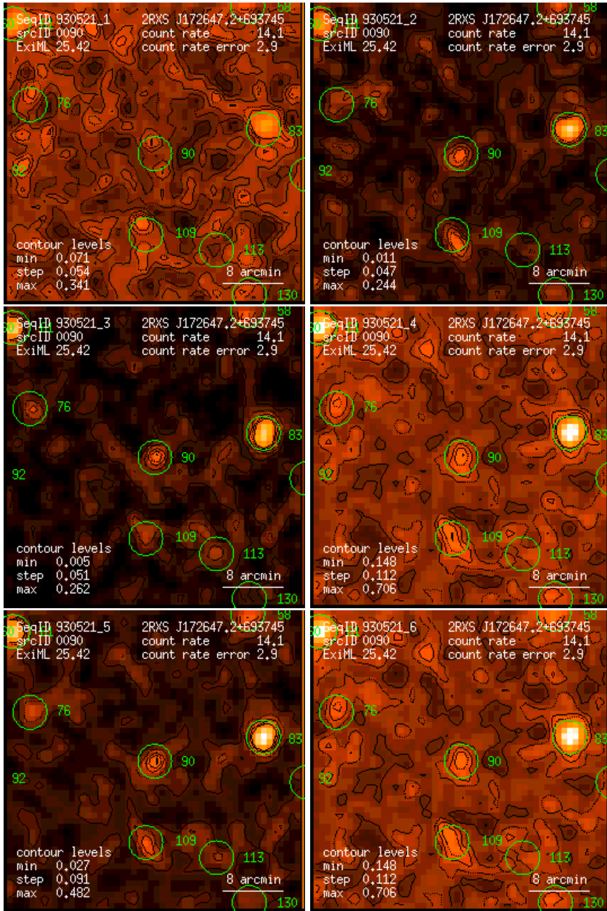
Figure 90: RASS 930521: detection 0090: band rate images, Gaussian filter: (1) PSPC channels 11 – 41, (2) 52 – 90, (3) 91 – 201, (4) 11 – 235, (5) 52 – 201, (6) 11 – 201. Broad band rates in counts/ks. Band rate contour levels in counts/ks/arcmin 2 .
