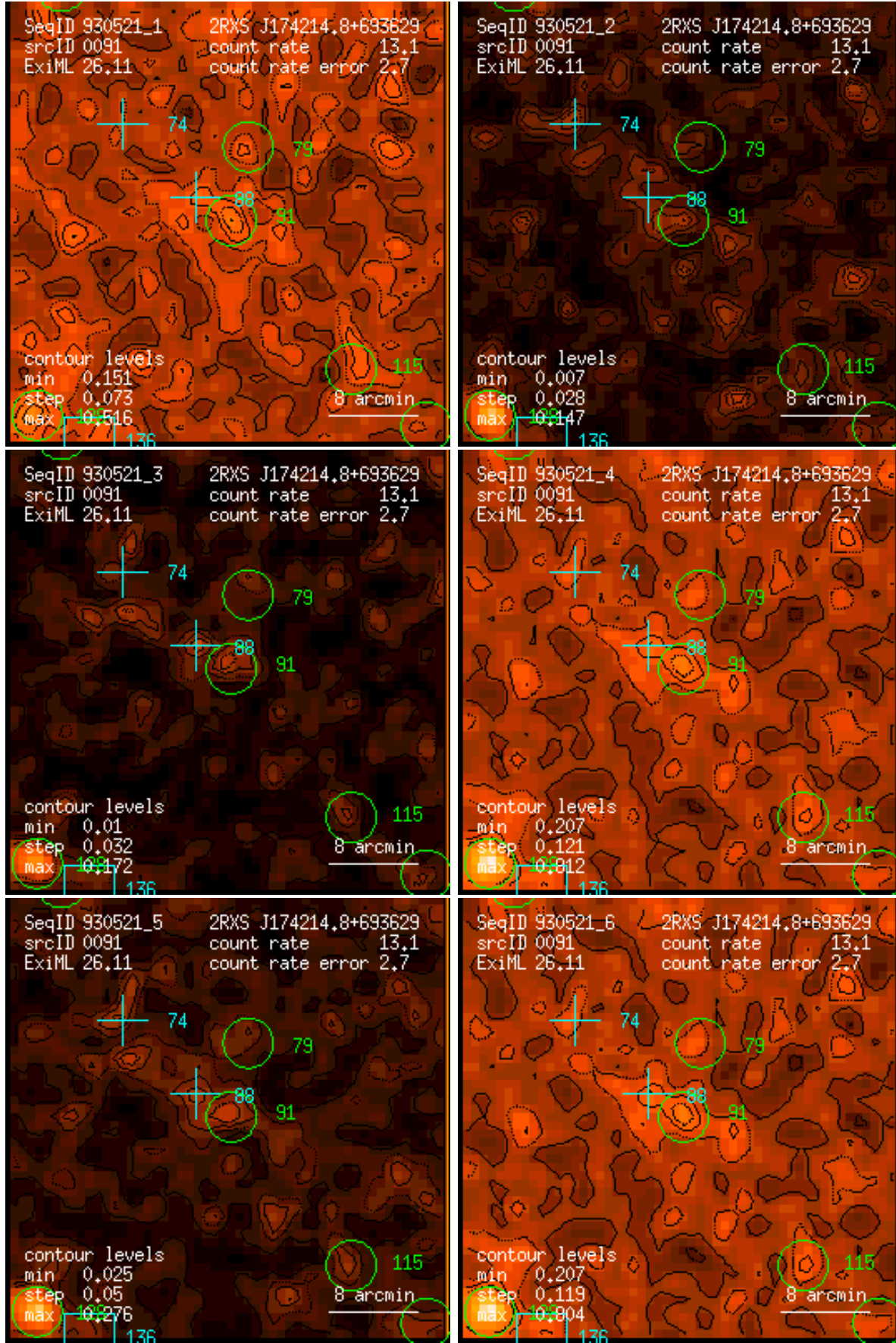
Figure 91: RASS 930521: detection 0091: band rate images, Gaussian filter: (1) PSPC channels 11 – 41, (2) 52 – 90, (3) 91 – 201, (4) 11 – 235, (5) 52 – 201, (6) 11 – 201. Broad band rates in counts/ks. Band rate contour levels in counts/ks/arcmin 2 .
