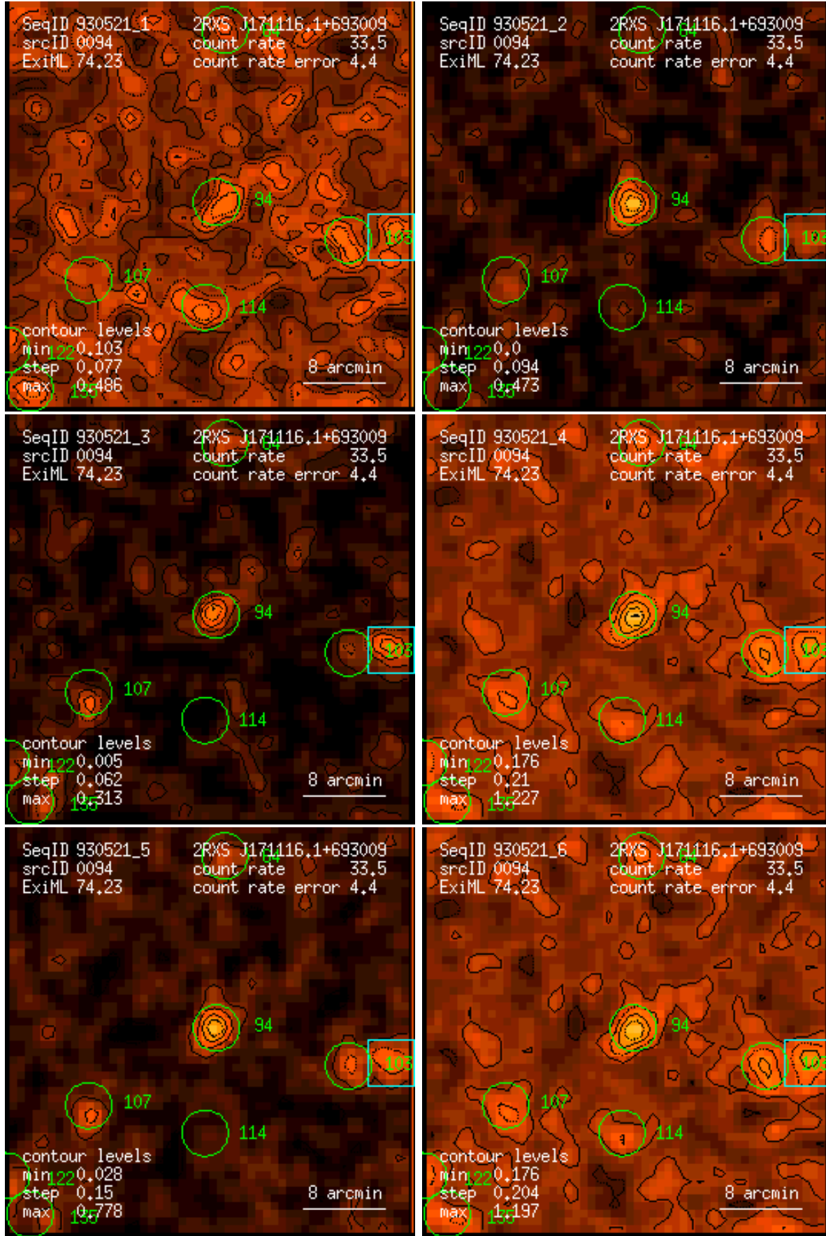
Figure 94: RASS 930521: detection 0094: band rate images, Gaussian filter: (1) PSPC channels 11 – 41, (2) 52 – 90, (3) 91 – 201, (4) 11 – 235, (5) 52 – 201, (6) 11 – 201. Broad band rates in counts/ks. Band rate contour levels in counts/ks/arcmin 2 .
