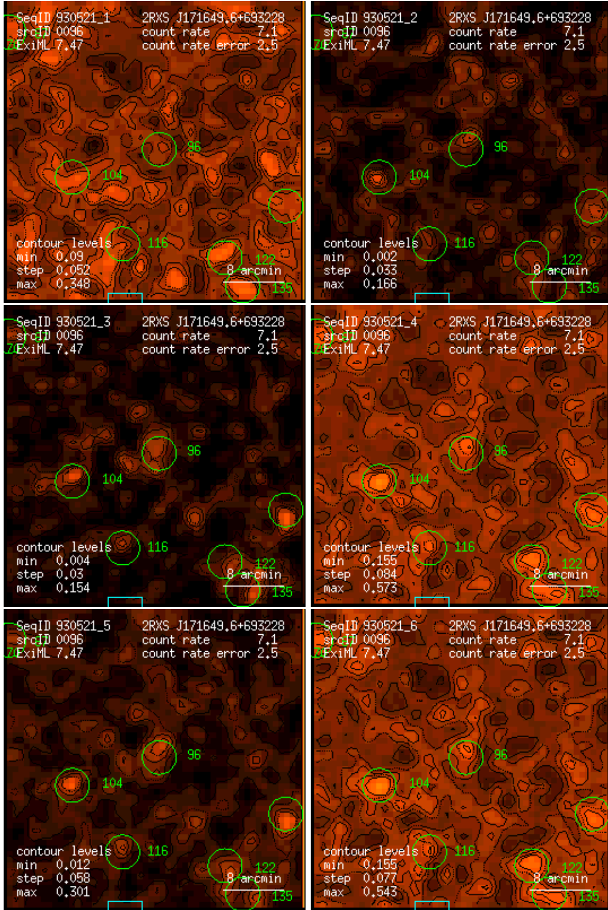
Figure 96: RASS 930521: detection 0096: band rate images, Gaussian filter: (1) PSPC channels 11 – 41, (2) 52 – 90, (3) 91 – 201, (4) 11 – 235, (5) 52 – 201, (6) 11 – 201. Broad band rates in counts/ks. Band rate contour levels in counts/ks/arcmin 2 .
