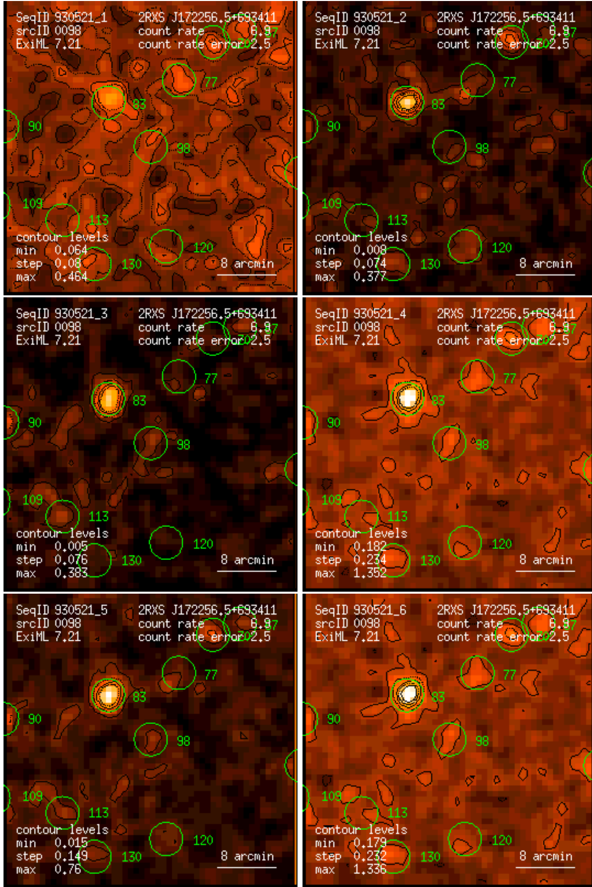
Figure 98: RASS 930521: detection 0098: band rate images, Gaussian filter: (1) PSPC channels 11 – 41, (2) 52 – 90, (3) 91 – 201, (4) 11 – 235, (5) 52 – 201, (6) 11 – 201. Broad band rates in counts/ks. Band rate contour levels in counts/ks/arcmin 2 .
