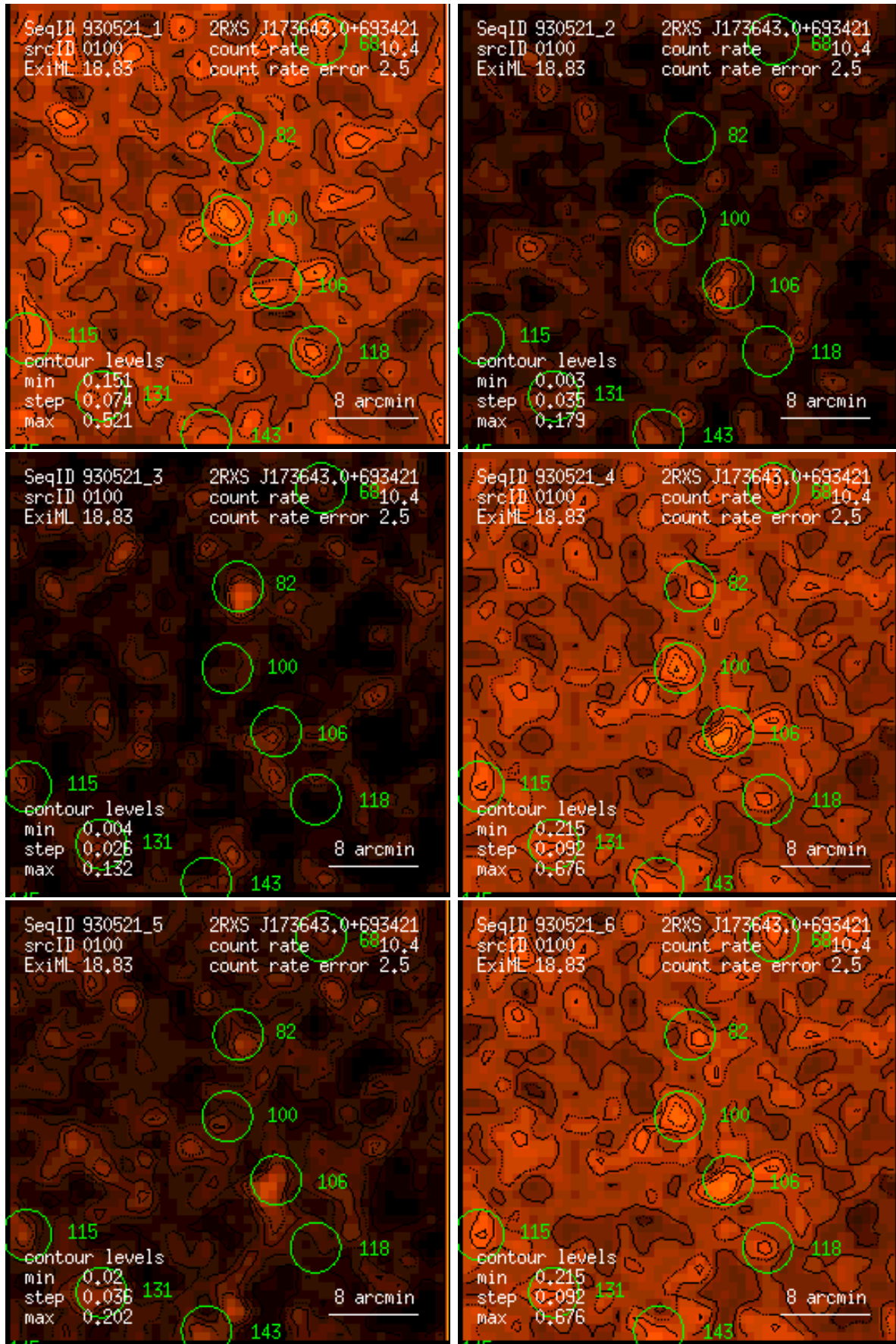
Figure 100: RASS 930521: detection 0100: band rate images, Gaussian filter: (1) PSPC channels 11 – 41, (2) 52 – 90, (3) 91 – 201, (4) 11 – 235, (5) 52 – 201, (6) 11 – 201. Broad band rates in counts/ks. Band rate contour levels in counts/ks/arcmin 2 .
