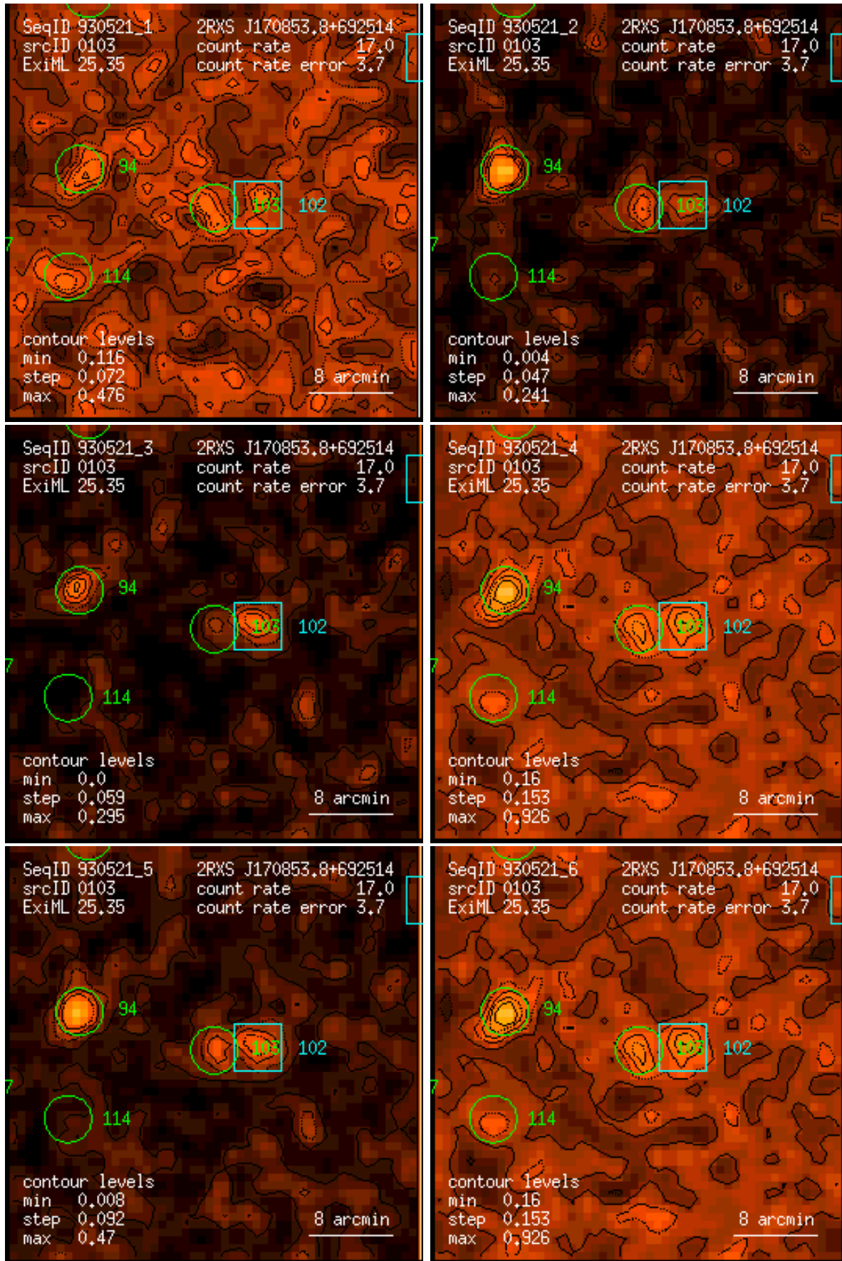
Figure 103: RASS 930521: detection 0103: band rate images, Gaussian filter: (1) PSPC channels 11 – 41, (2) 52 – 90, (3) 91 – 201, (4) 11 – 235, (5) 52 – 201, (6) 11 – 201. Broad band rates in counts/ks. Band rate contour levels in counts/ks/arcmin 2 .
