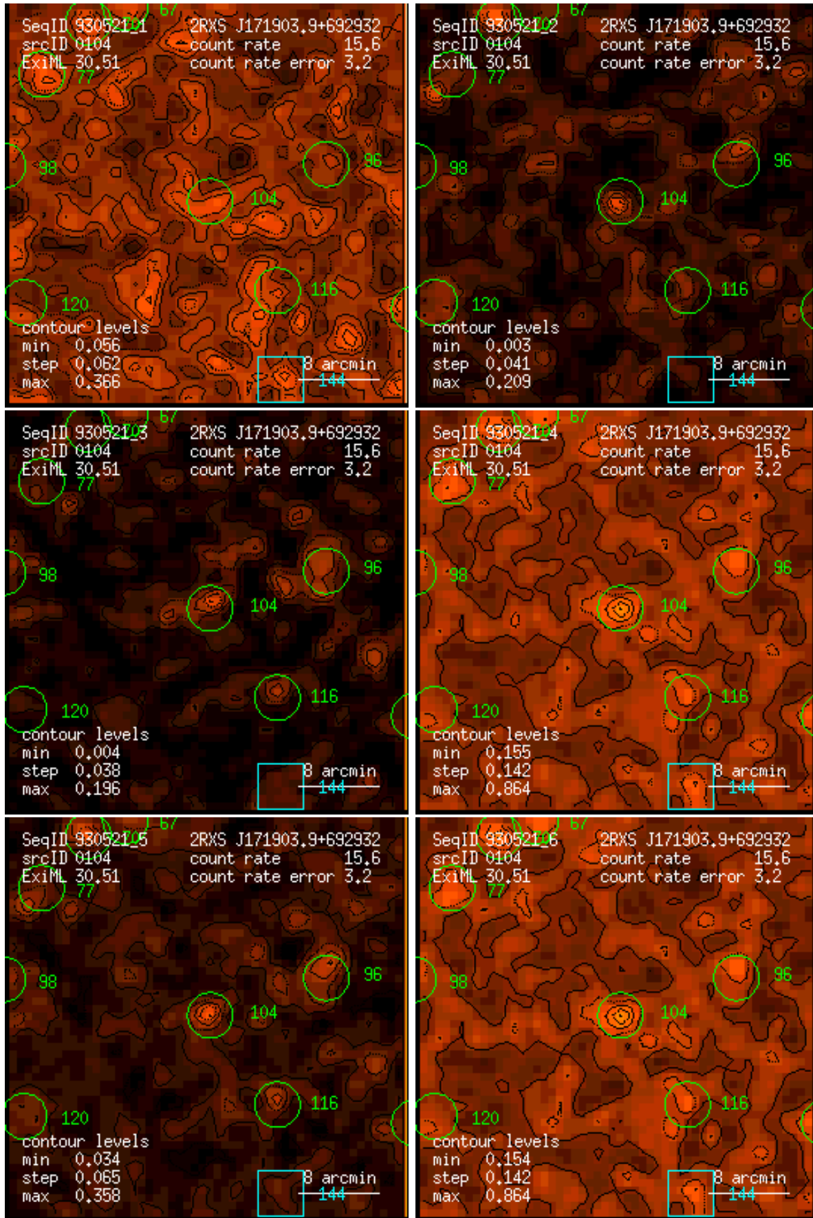
Figure 104: RASS 930521: detection 0104: band rate images, Gaussian filter: (1) PSPC channels 11 – 41, (2) 52 – 90, (3) 91 – 201, (4) 11 – 235, (5) 52 – 201, (6) 11 – 201. Broad band rates in counts/ks. Band rate contour levels in counts/ks/arcmin 2 .
