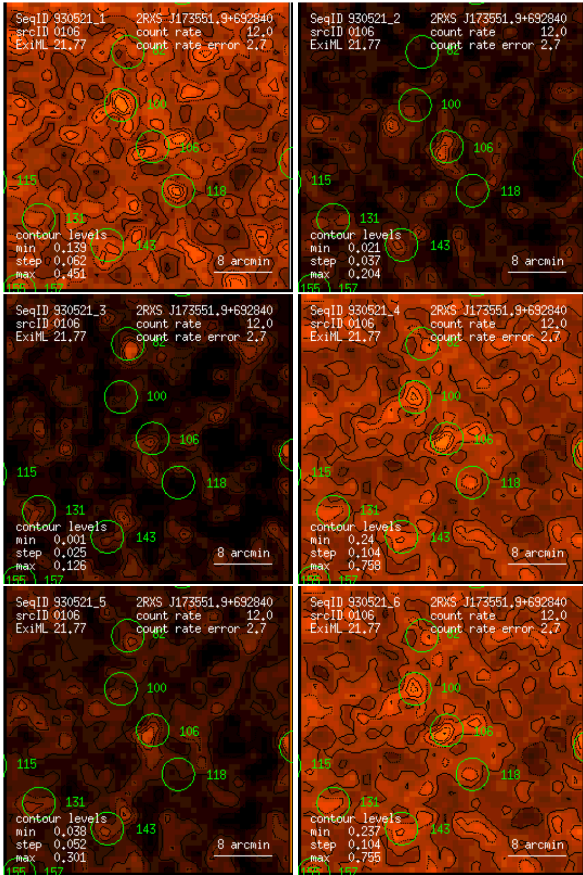
Figure 106: RASS 930521: detection 0106: band rate images, Gaussian filter: (1) PSPC channels 11 – 41, (2) 52 – 90, (3) 91 – 201, (4) 11 – 235, (5) 52 – 201, (6) 11 – 201. Broad band rates in counts/ks. Band rate contour levels in counts/ks/arcmin 2 .
