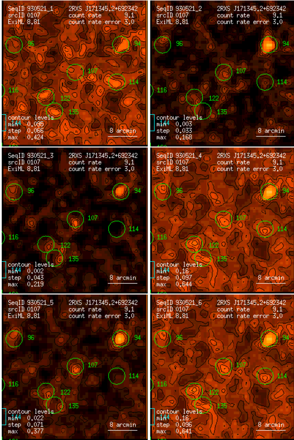
Figure 107: RASS 930521: detection 0107: band rate images, Gaussian filter: (1) PSPC channels 11 – 41, (2) 52 – 90, (3) 91 – 201, (4) 11 – 235, (5) 52 – 201, (6) 11 – 201. Broad band rates in counts/ks. Band rate contour levels in counts/ks/arcmin 2 .
